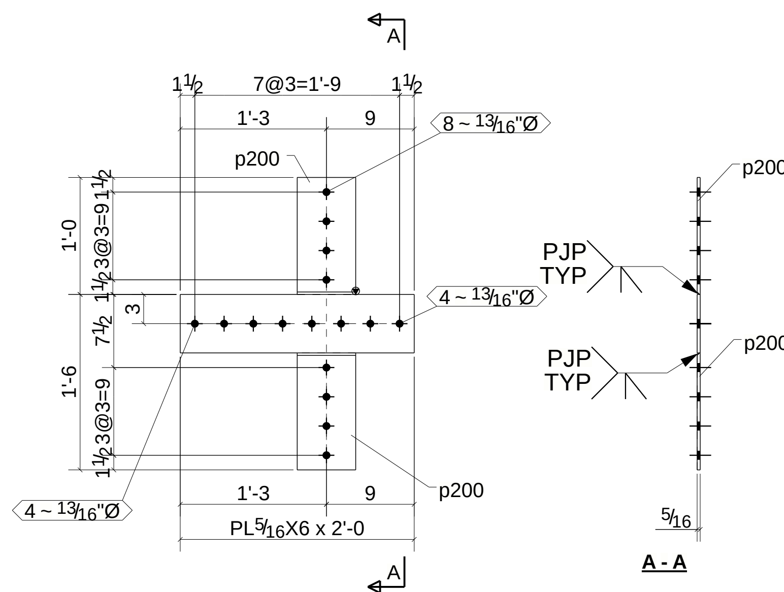
ONE - DRAG PLATE - 646PL6
