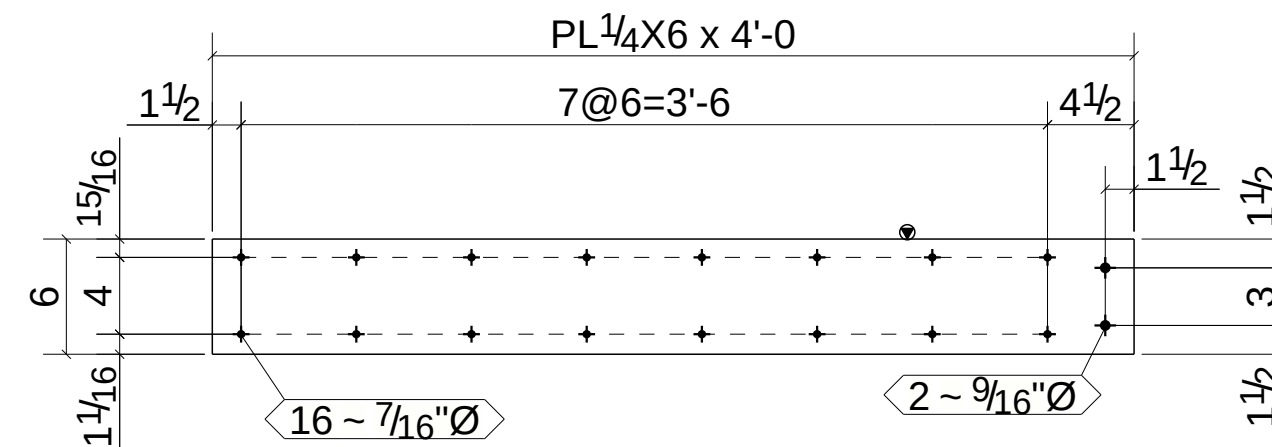
ONE - DRAG PLATE - 646PL2
