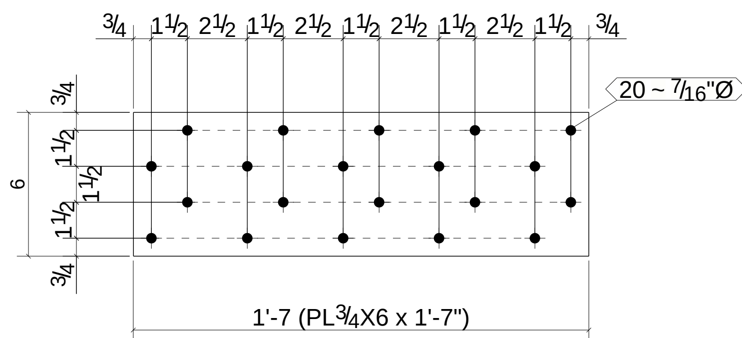
ONE - END PLATE - 646PL7
