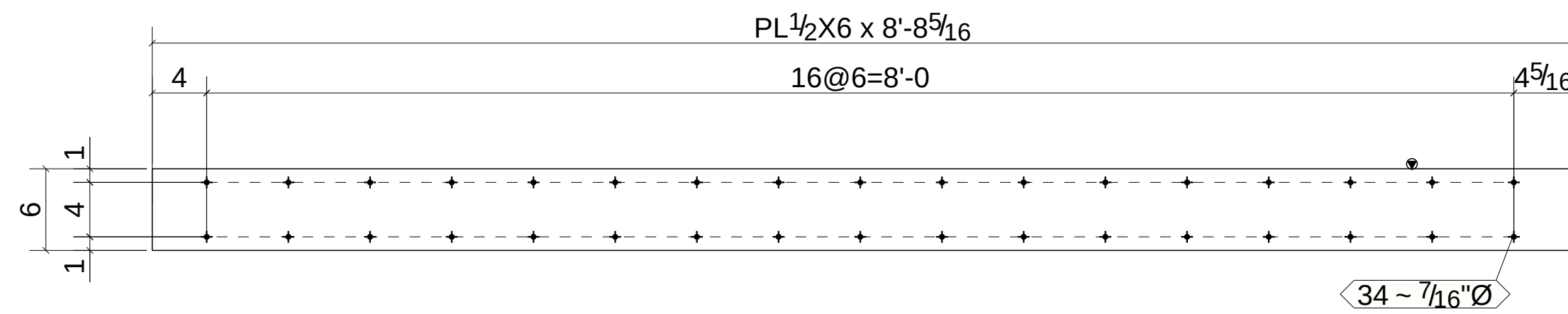
ONE - DRAG PLATE - 646PL1
