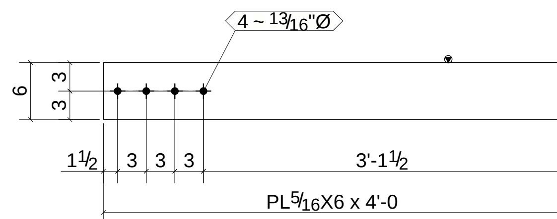
ONE - DRAG PLATE - 646PL5
