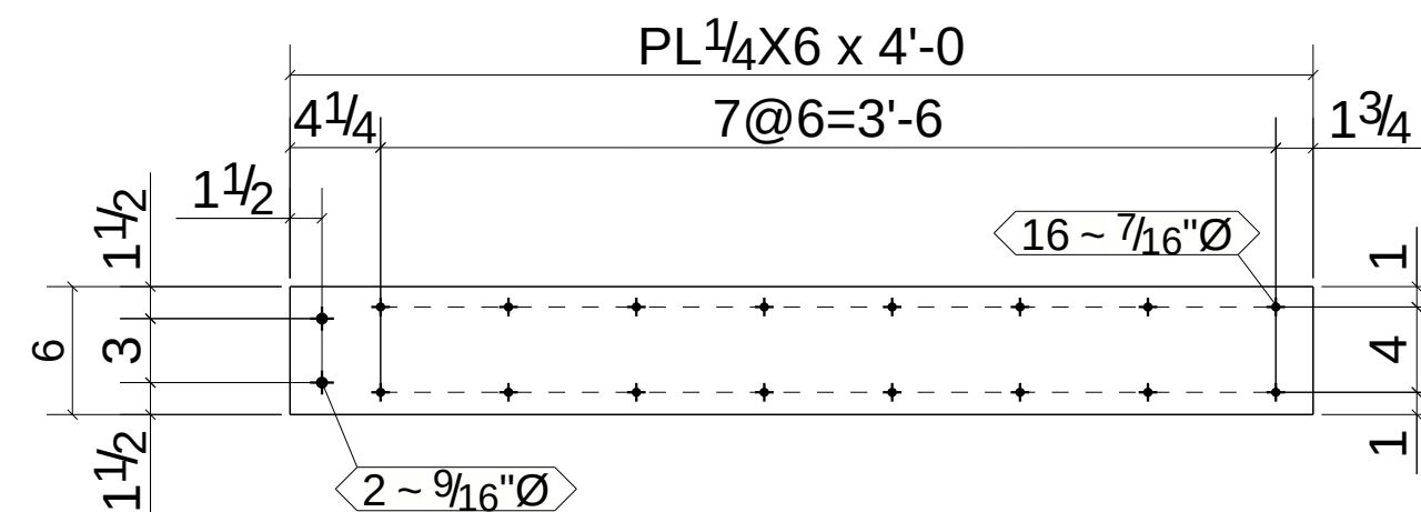
ONE - DRAG PLATE - 646PL8
