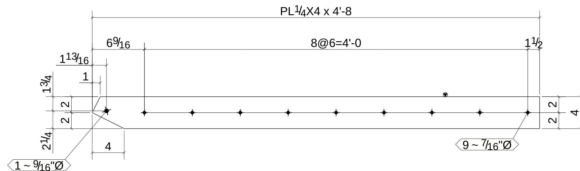
2 - DRAG PLATES - 646PL4
