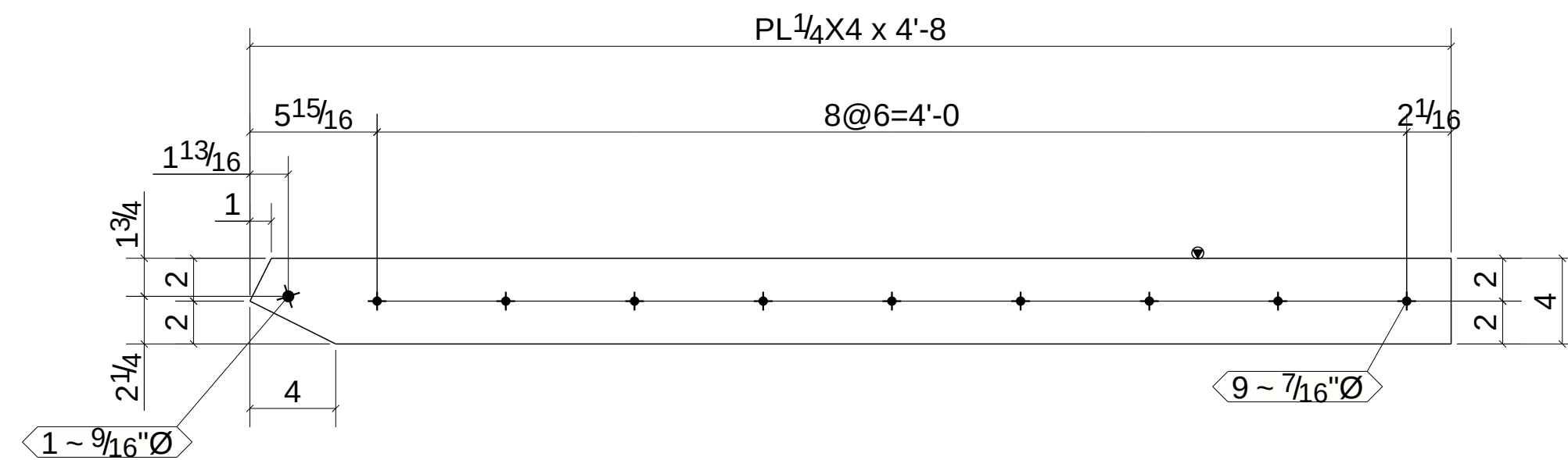
4 - DRAG PLATES - 646PL3
