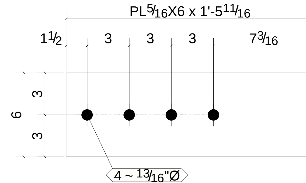
ONE - SPLICE PLATE - 648PL3
