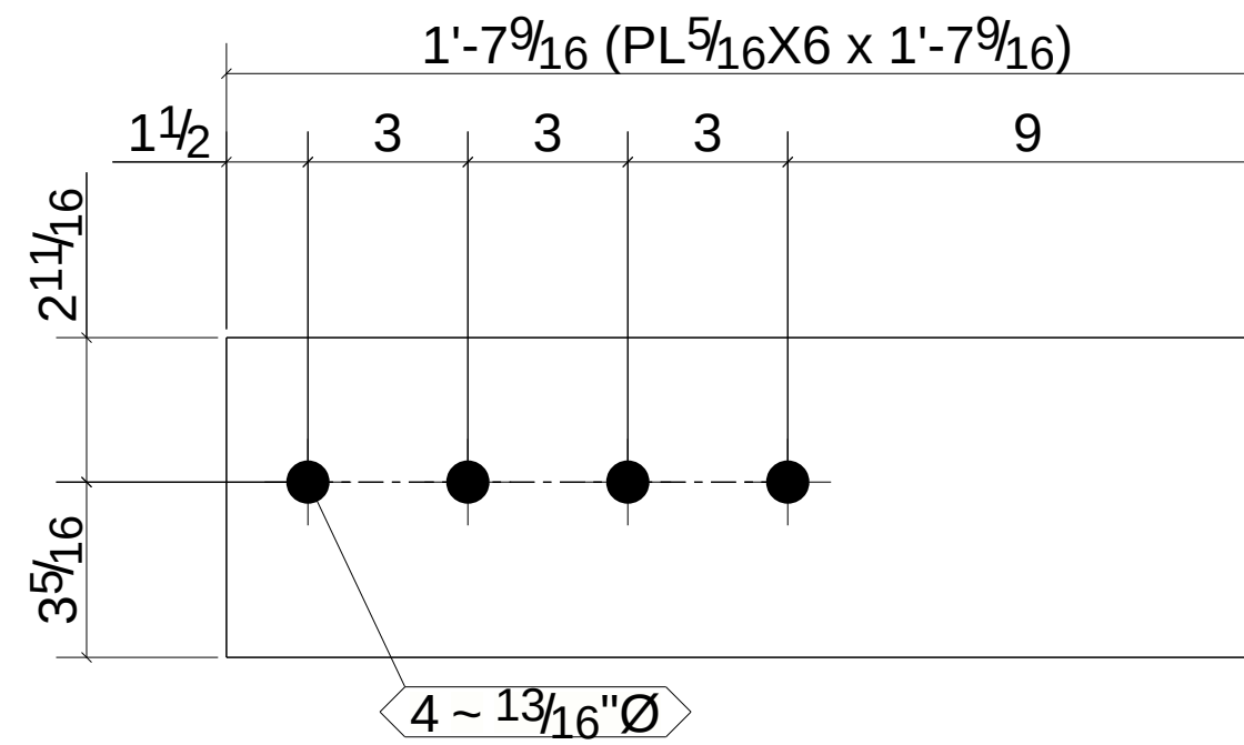
ONE - SPLICE PLATE - 648PL2
