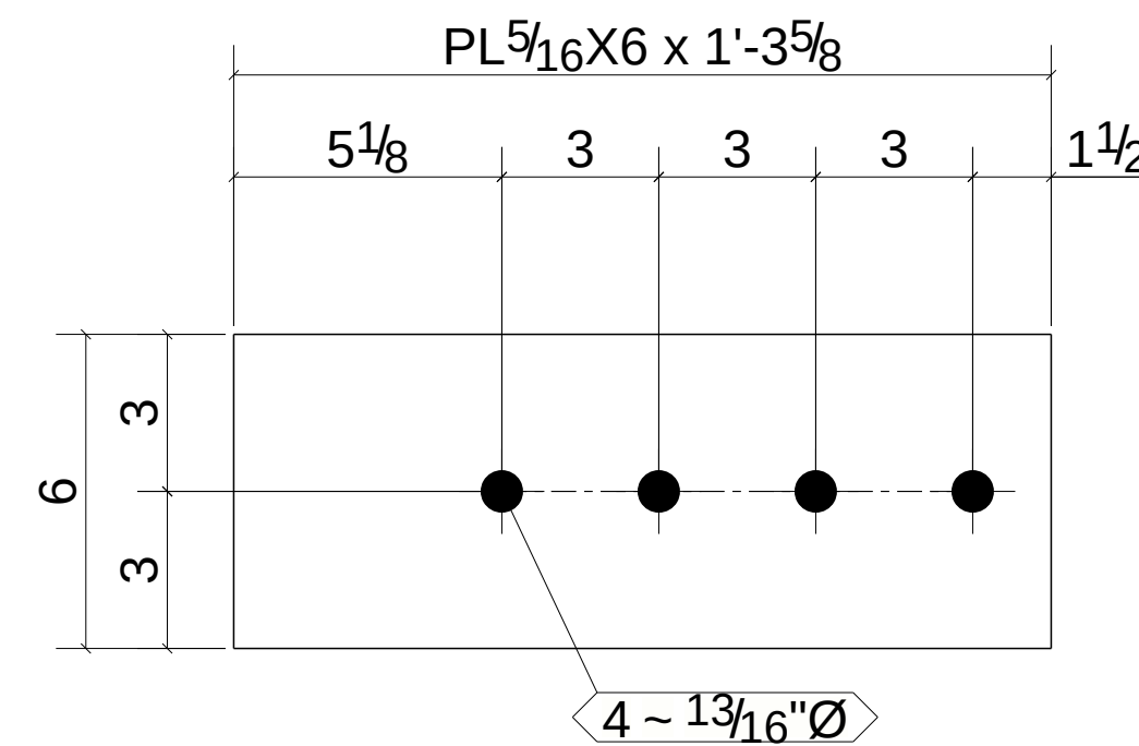
ONE - SPLICE PLATE - 648PL4
