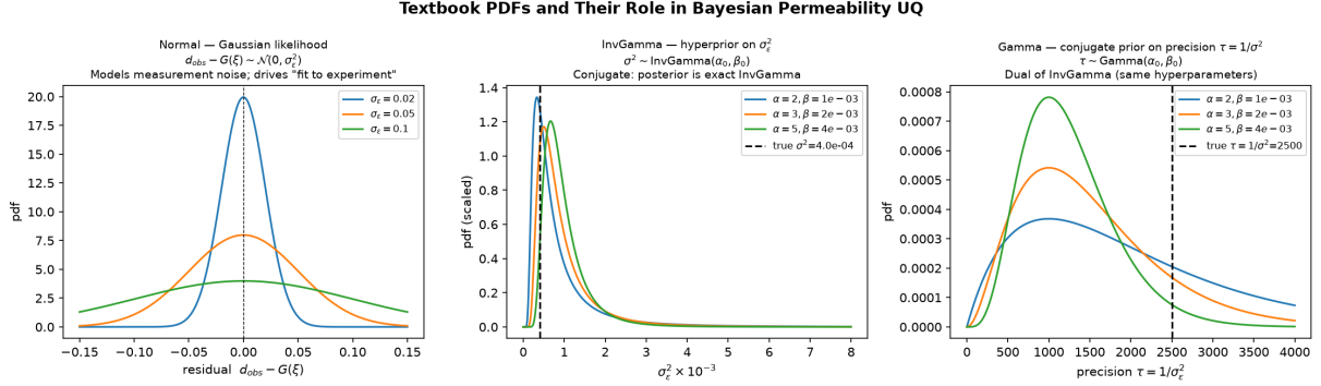
Figure 1: The three foundational distributions for Gaussian-likelihood UQ. Left: Normal—models measurement noise and the log-permeability prior. Centre: Inverse-Gamma—conjugate hyperprior on the noise variance \sigma_\varepsilon^2 . Right: Gamma—conjugate prior on the precision \tau = 1/\sigma_\varepsilon^2 .
