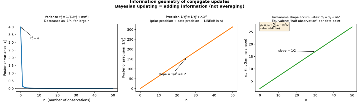
Figure 7: Information geometry of conjugate updates. Left: posterior variance \tau_n^2 decreases hyperbolically in n . Centre: posterior precision 1/\tau_n^2 is linear in n (information adds). Right: InvGamma shape parameter \alpha_n = \alpha_0 + n/2 is also linear (“half-observation” accumulation).
