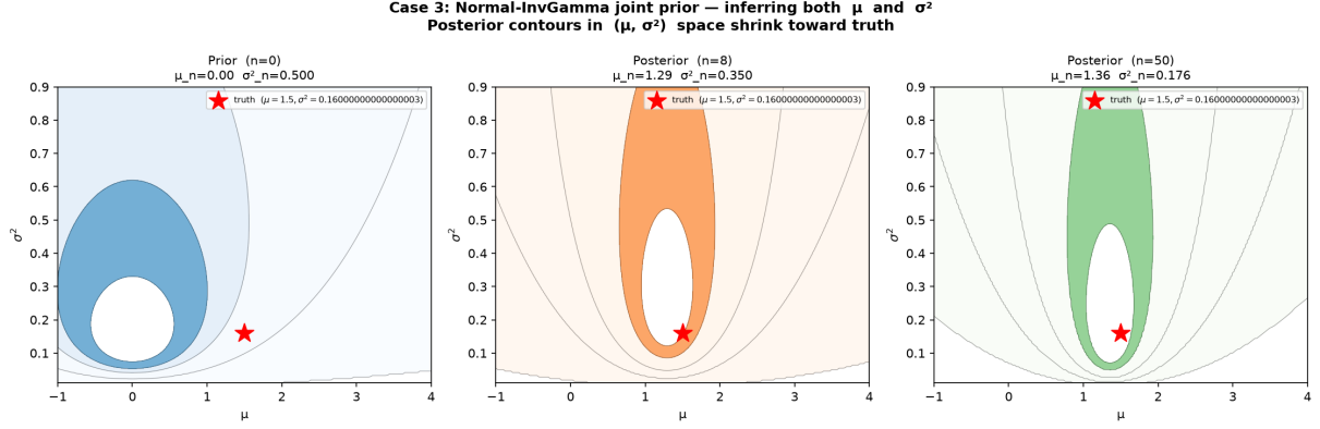
Figure 8: Joint NIG posterior contours in (\mu, \sigma^2) space. Left : the prior spans a wide region. Centre : after n = 8 observations, the contours begin to concentrate. Right : after n = 50 , the posterior is a tight ellipse around the true values (red star).
