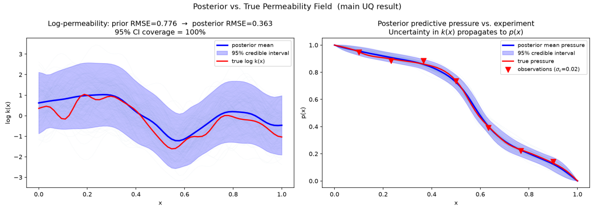
Figure 11: Posterior vs. true permeability field. Left: log-permeability posterior mean (blue), 95% pointwise credible interval (shaded), and true field (red). The prior RMSE (mean field vs. truth) of 0.78 is reduced to 0.36 in the posterior. Coverage of the 95% CI is \approx 100\% for this case, indicating slight over-coverage from the Gibbs-inferred noise variance. Right: posterior predictive pressure compared to the noisy observations. The uncertainty in k(x) propagates to uncertainty in p(x) .
