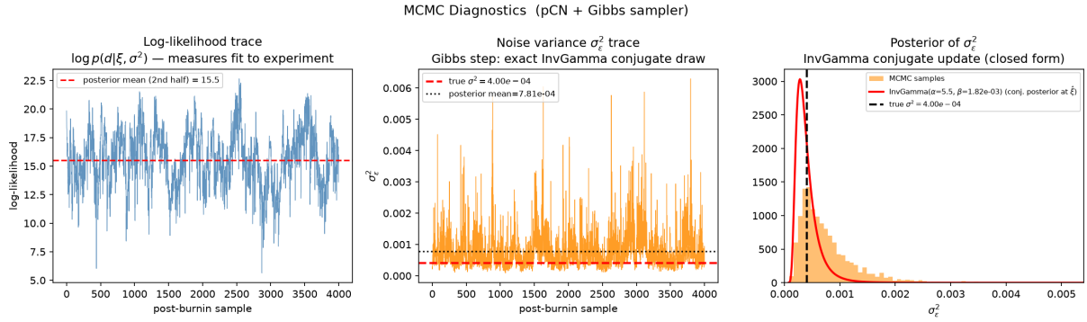
Figure 10: pCN-Gibbs MCMC diagnostics. Left: log-likelihood trace shows rapid mixing after the burn-in period. Centre: noise variance \sigma_\epsilon^2 trace mixes around the true value (red dashed). Right: posterior histogram of \sigma_\epsilon^2 overlaid with the analytical InvGamma posterior at the posterior-mean \xi , demonstrating that the Gibbs step is correctly implemented.
