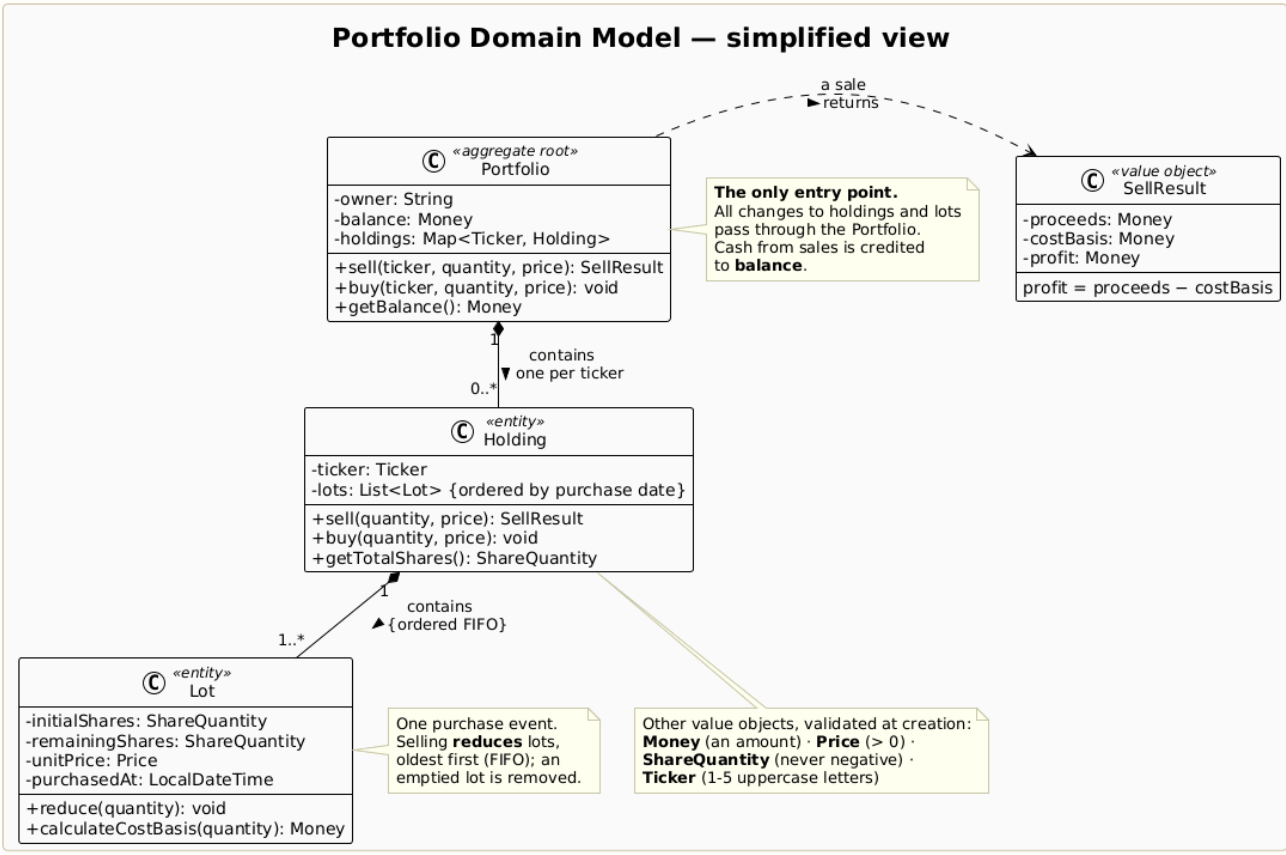
Domain model — Portfolio, Holding, Lot and the value objects
