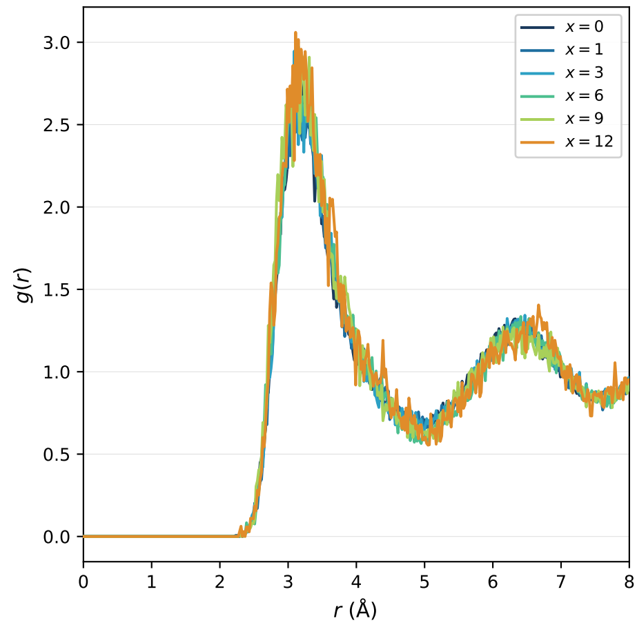
g(r) — Ca-Na
