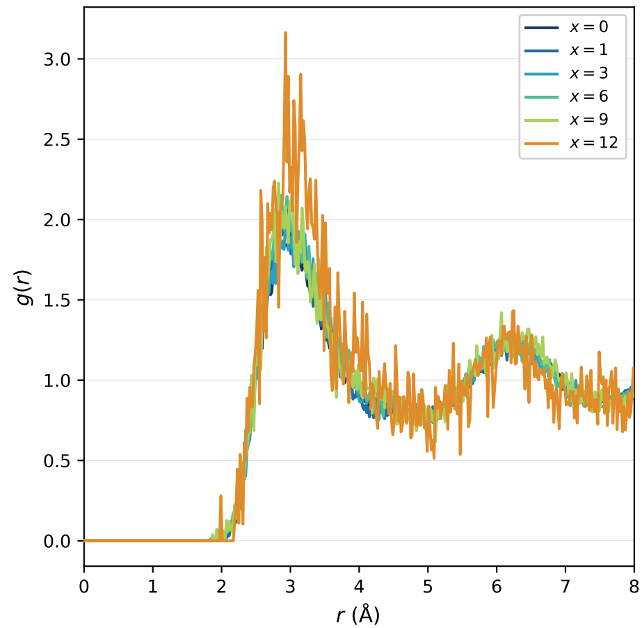
g(r) — Na-Na
