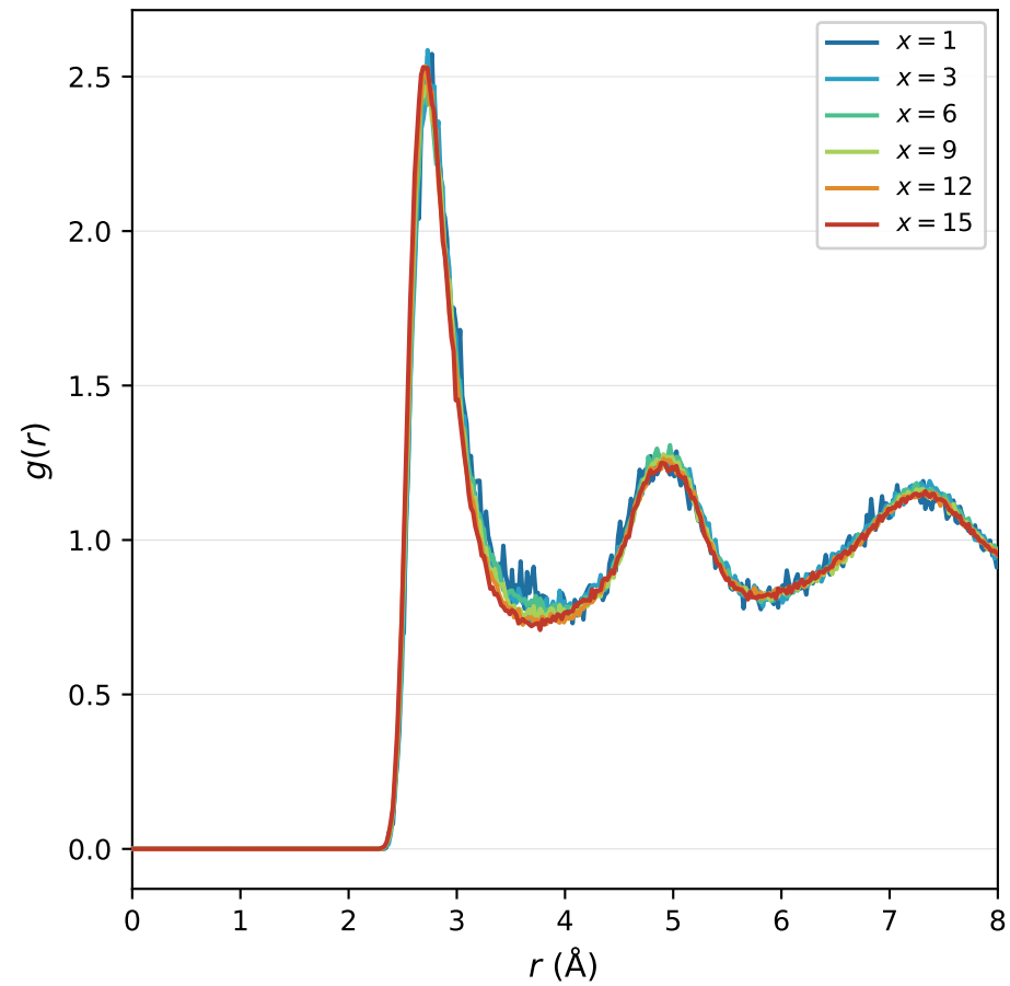
g(r) — O-K
