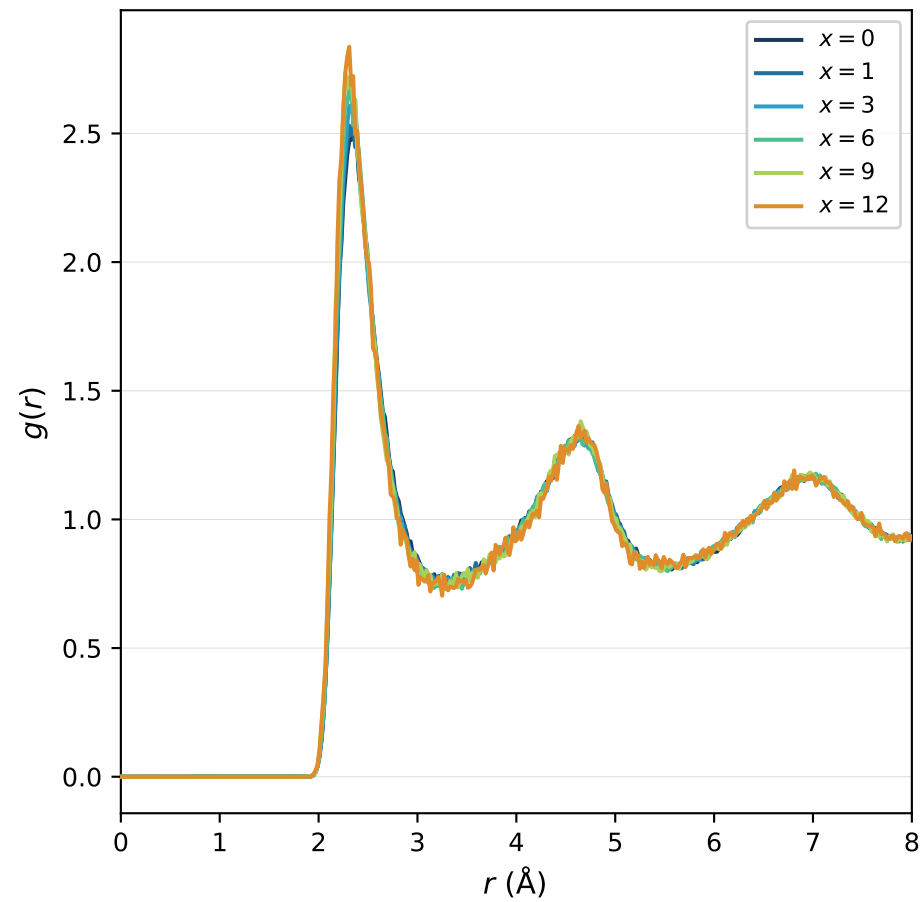
g(r) — O-Na
