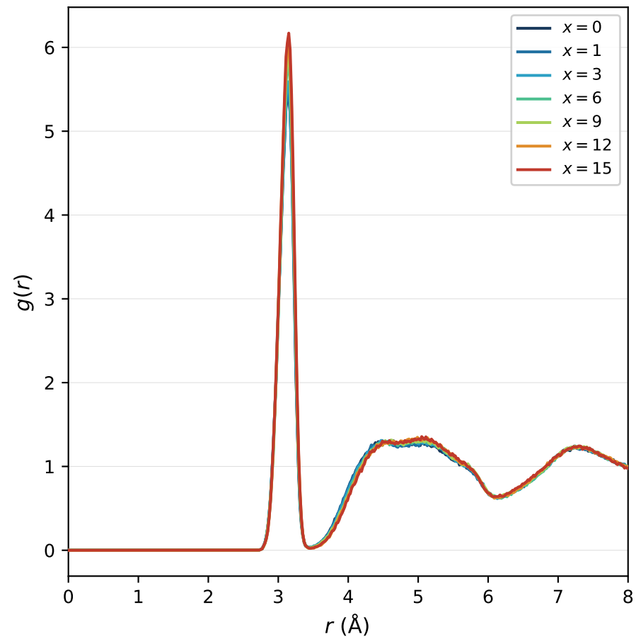
g(r) — Si-Si
