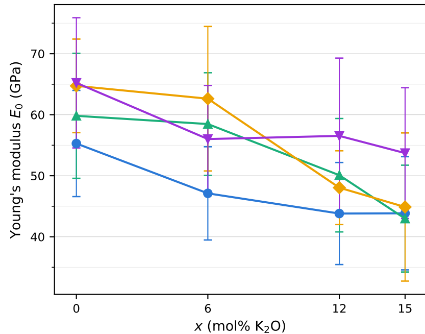
PMMCS — Young's modulus (stress-strain) and Bulk modulus (pressure ramp) 75\text{SiO}_2 \cdot (15-x)\text{Na}_2\text{O} \cdot x\text{K}_2\text{O} \cdot 10\text{CaO} , 300 K
