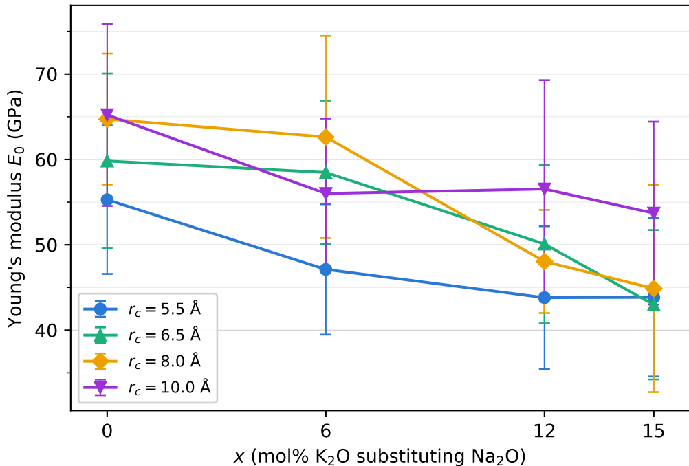
PMMCS: Young's modulus via stress-strain 75\text{SiO}_2 \cdot (15-x)\text{Na}_2\text{O} \cdot x\text{K}_2\text{O} \cdot 10\text{CaO} , 300 K
