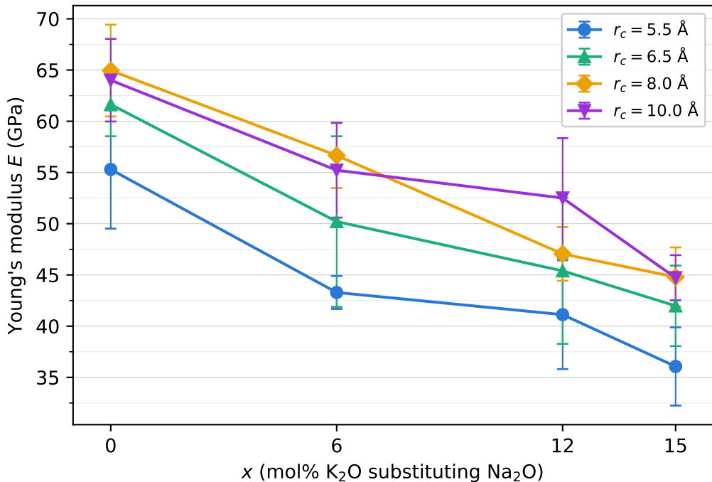
PMMCS: Young's modulus vs composition 75\text{SiO}_2 \cdot (15-x)\text{Na}_2\text{O} \cdot x\text{K}_2\text{O} \cdot 10\text{CaO}
