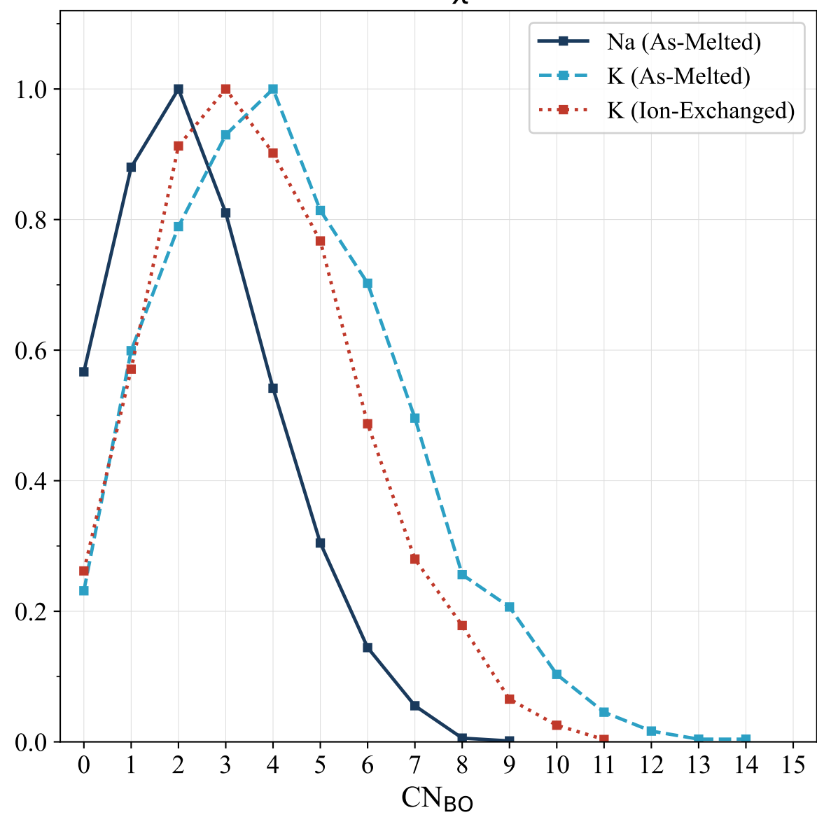
Ca-free — \chi = 20\%
