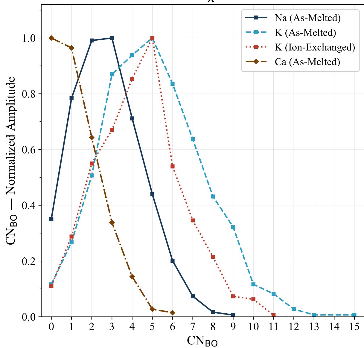
10CaO — \chi = 20\%
