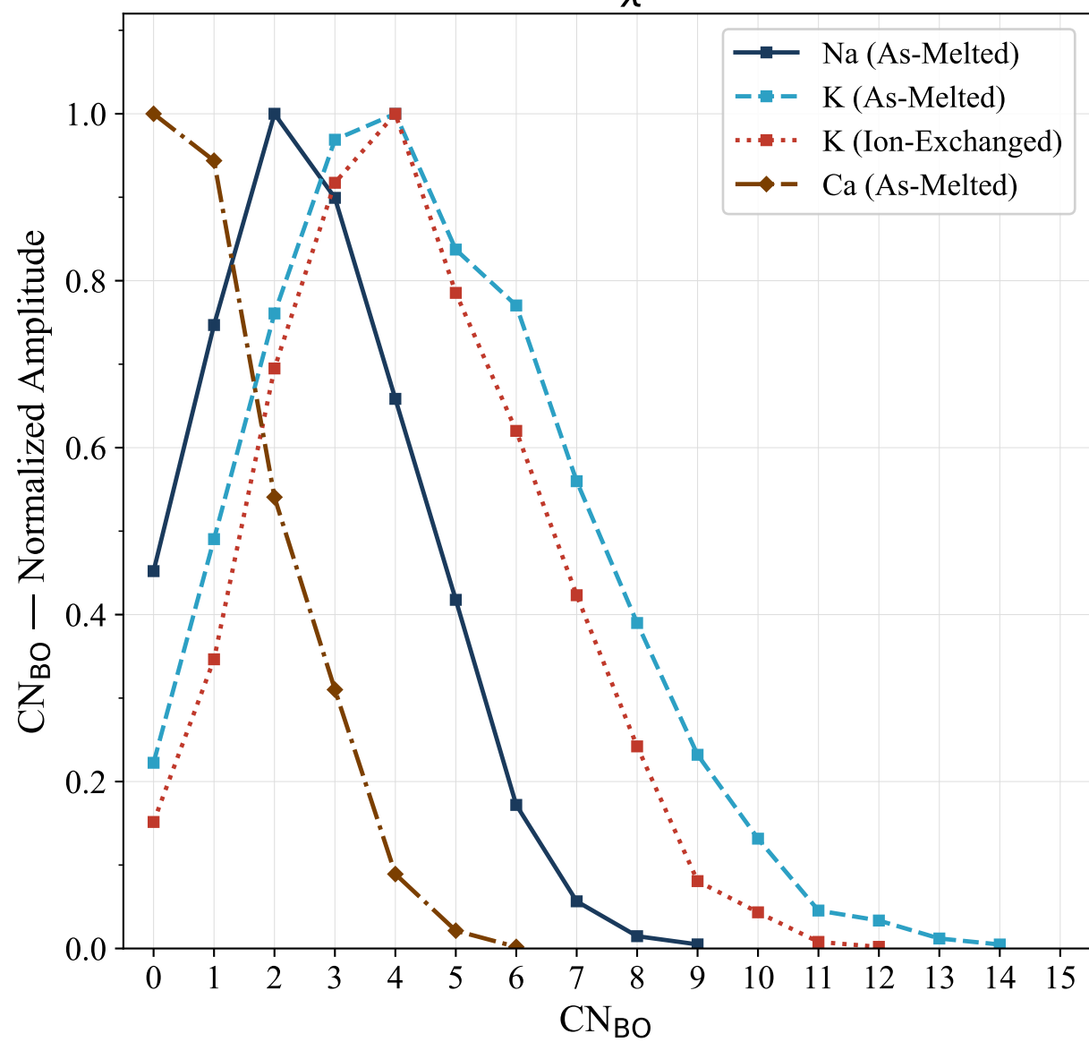
10CaO — \chi = 60\%
