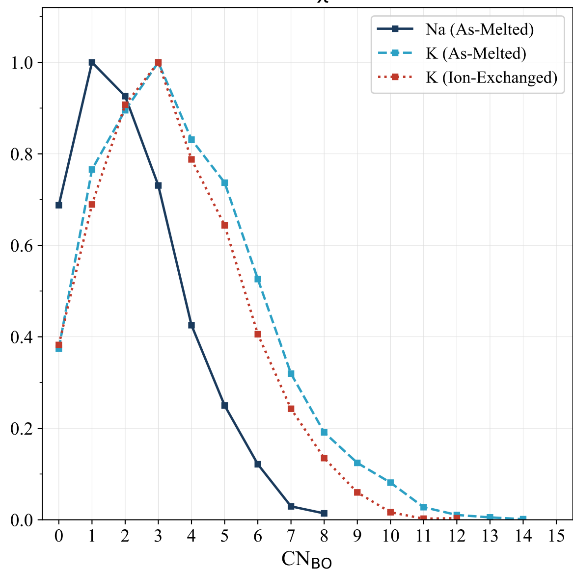
Ca-free — \chi = 60\%
