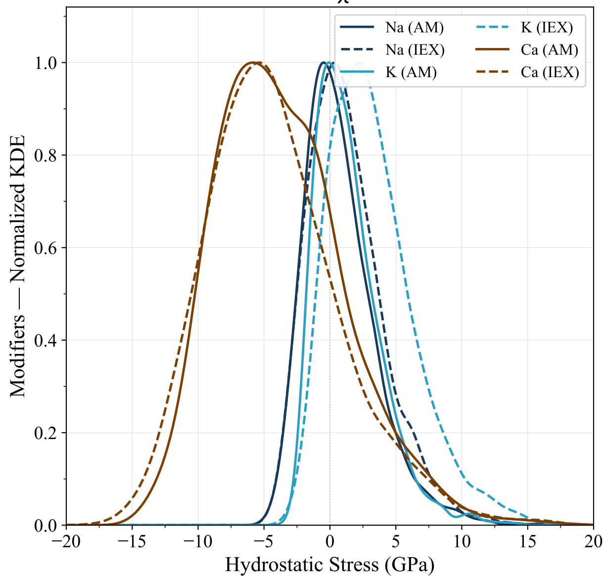
10CaO — \chi = 60\%
