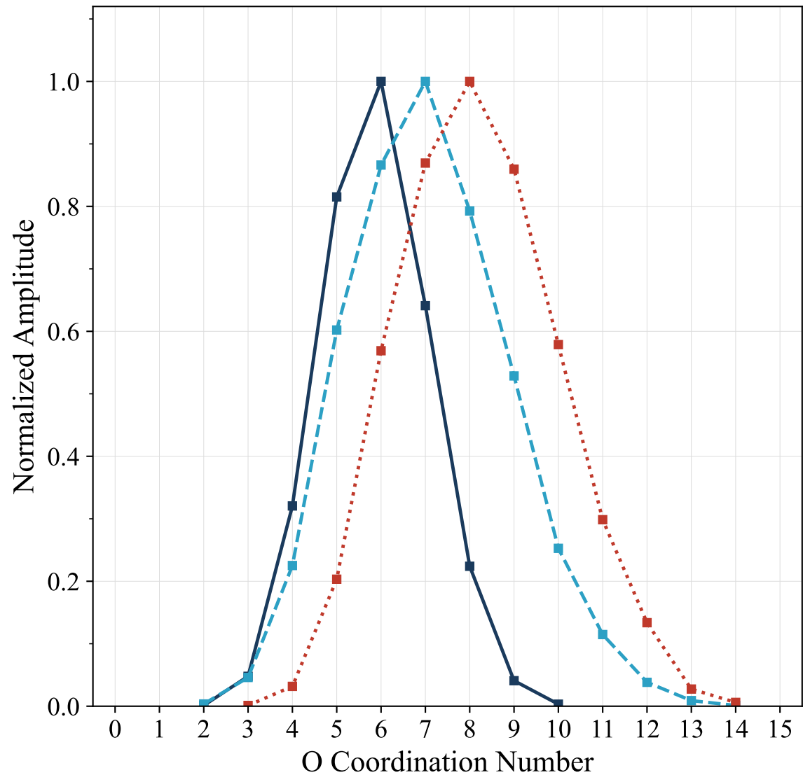
Ca-free — \chi = 100\%
