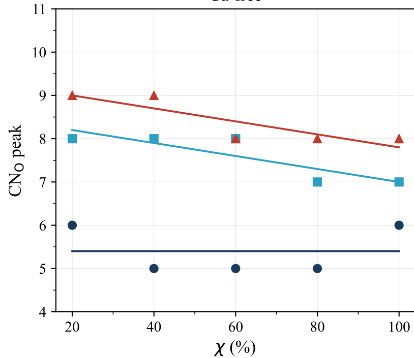
Ca-free
