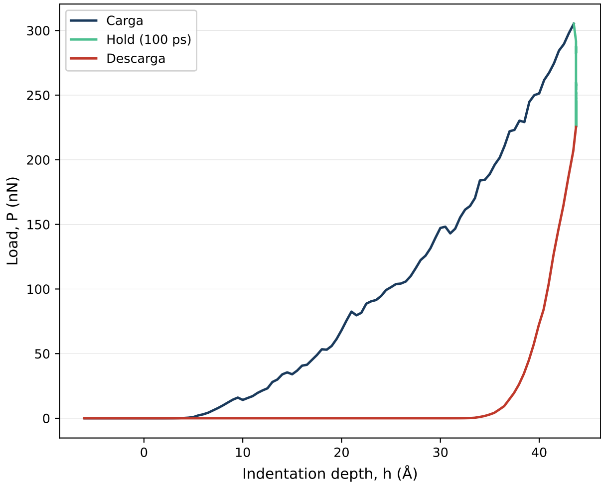
Nanoindentation P-h curve — CaO x=0 r=1 (AM)
