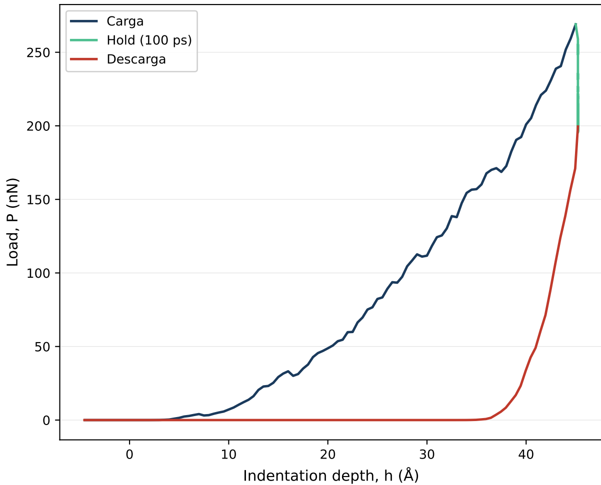
Nanoindentation P-h curve — sin-Ca x=0 r=1 (AM)
