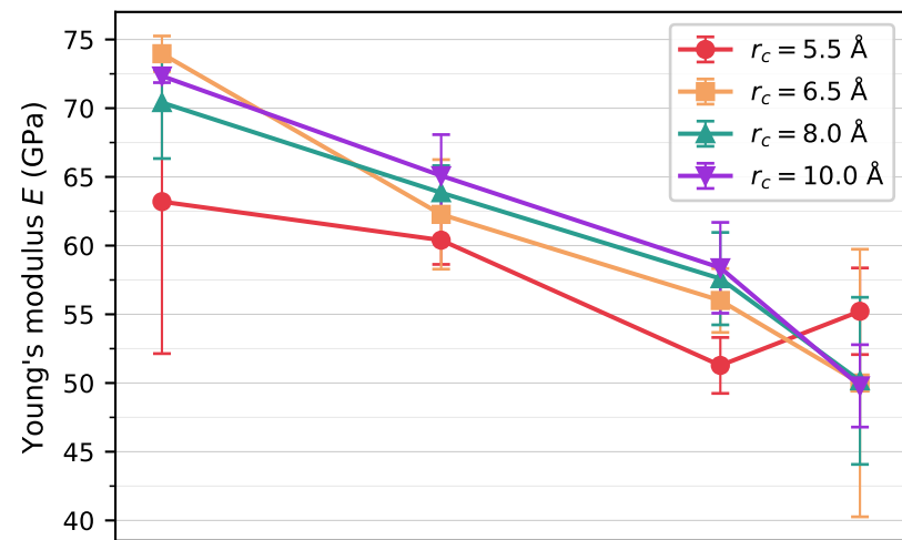
PMMCS — Elastic properties vs. short-range cutoff r_c , athermal ( T = 0 K) 75\text{SiO}_2 \cdot (15-x)\text{Na}_2\text{O} \cdot x\text{K}_2\text{O} \cdot 10\text{CaO}
