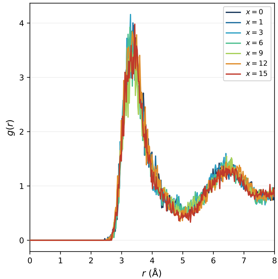
g(r) — Ca-Ca
