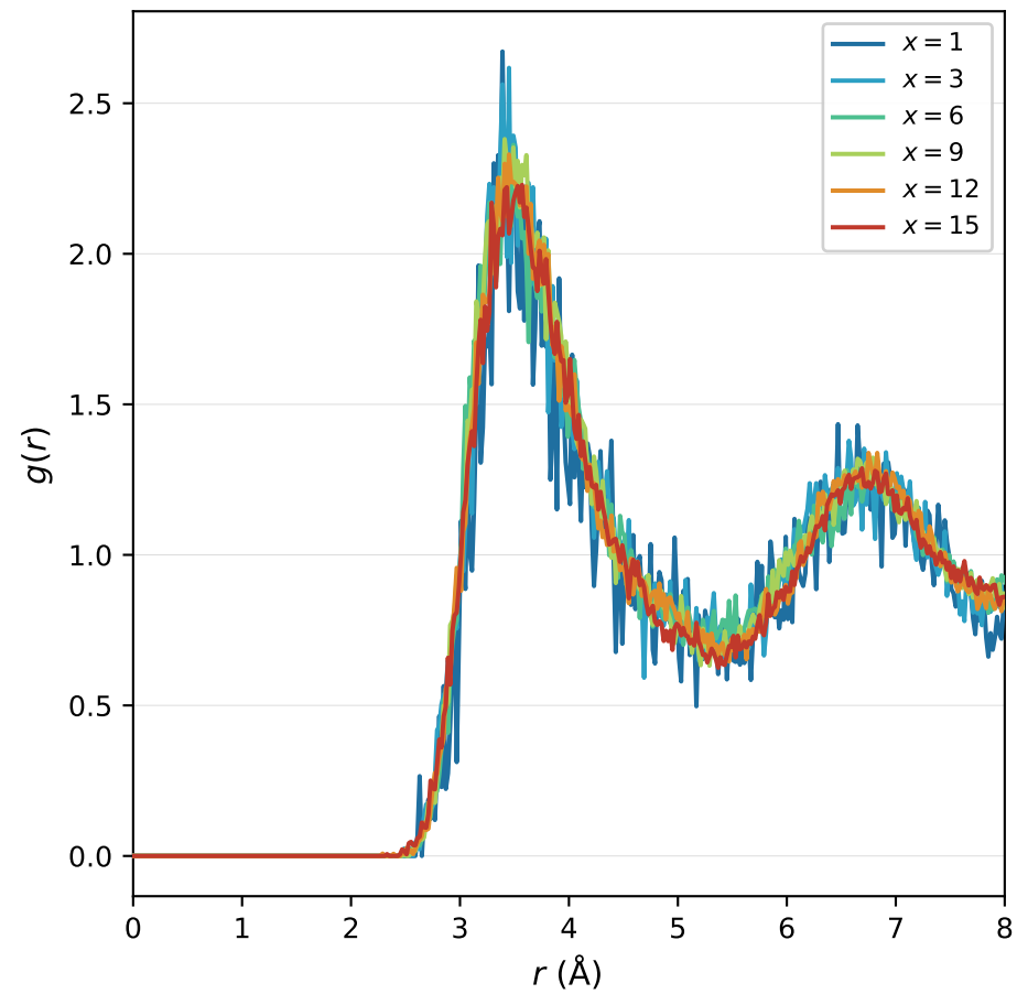
g(r) — Ca-K
