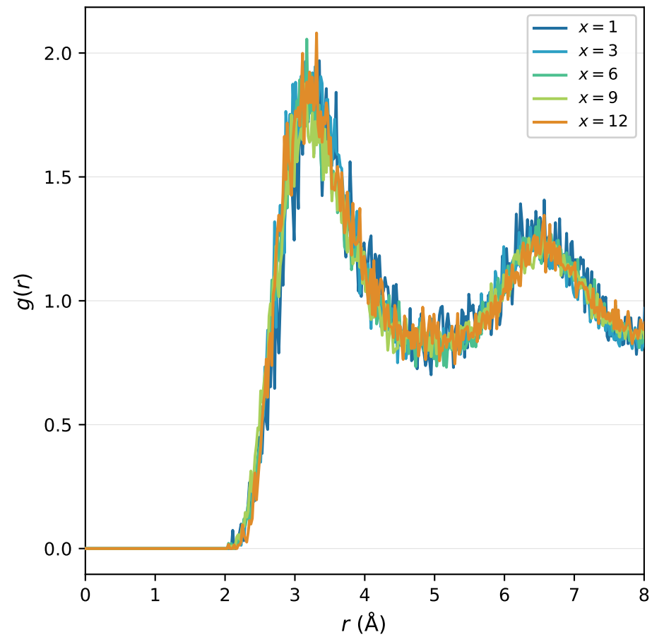
g(r) — Na-K
