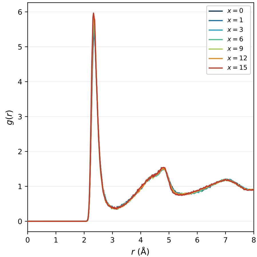
g(r) — O-Ca
