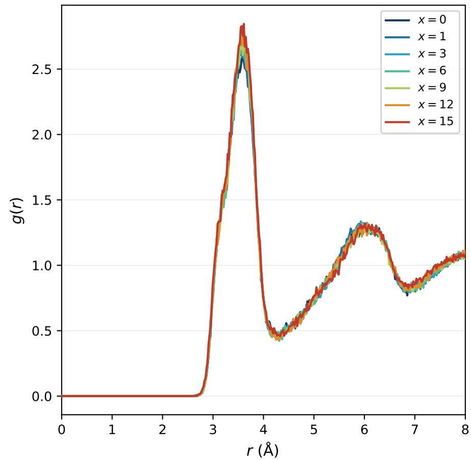
g(r) — Si-Ca
