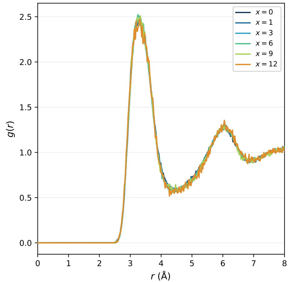
g(r) — Si-Na
