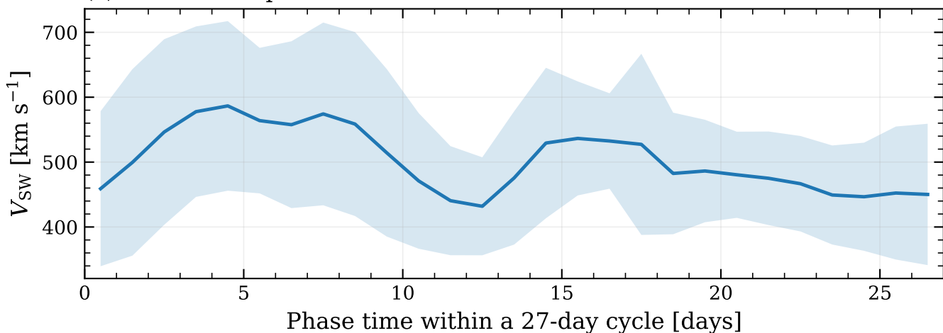
(c) Solar-wind speed
