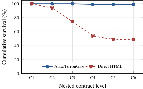
Figure 2: Nested contract survival on the main benchmark. C1: answer; C2: load; C3: reachable interaction; C4: bidirectional feedback; C5: hint, answer reveal, and log; C6: noninterference. Values are cumulative, not independent per-contract accuracies.
