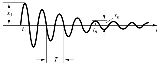
Figure 5-73 Decaying oscillation.
