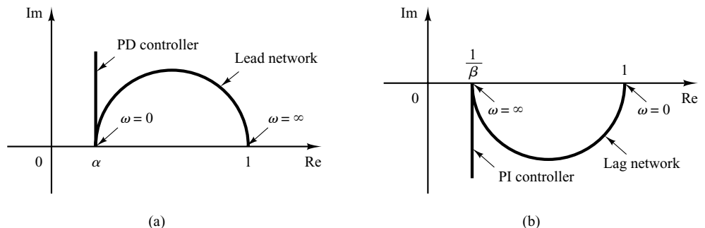
Figure 7–137 (a) Polar plots of a lead network and a proportional-plus-derivative controller; (b) polar plots of a lag network and a proportional-plus-integral controller.
