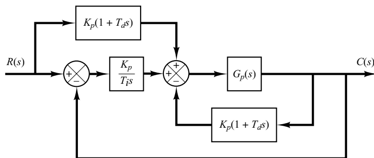
Figure 8-72 (a) PID-controlled system; (b) I-PD-controlled system with feedforward control.
