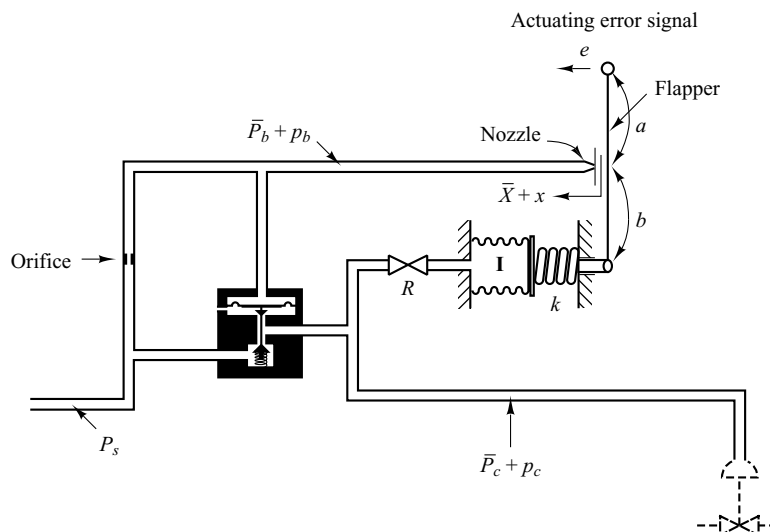
Figure 4-46 Pneumatic controller.
