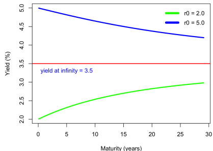
Yield Curves Under the Vasicek Model
