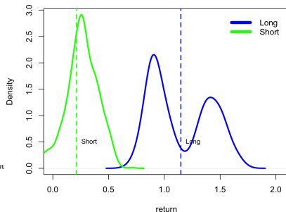
Return Distributions for Long and Short Holding Periods
