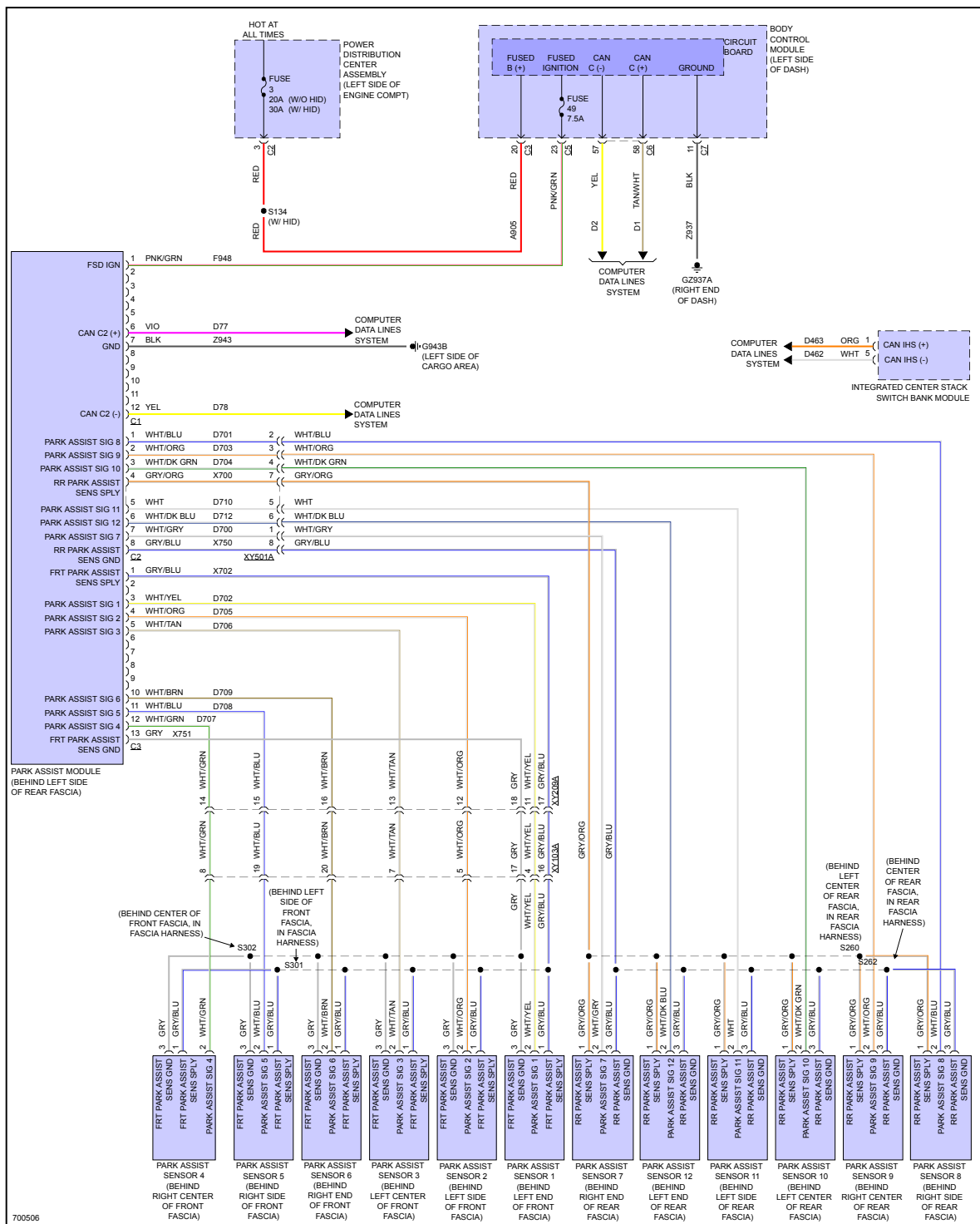
Fig 7: Parking Assistant Circuit
