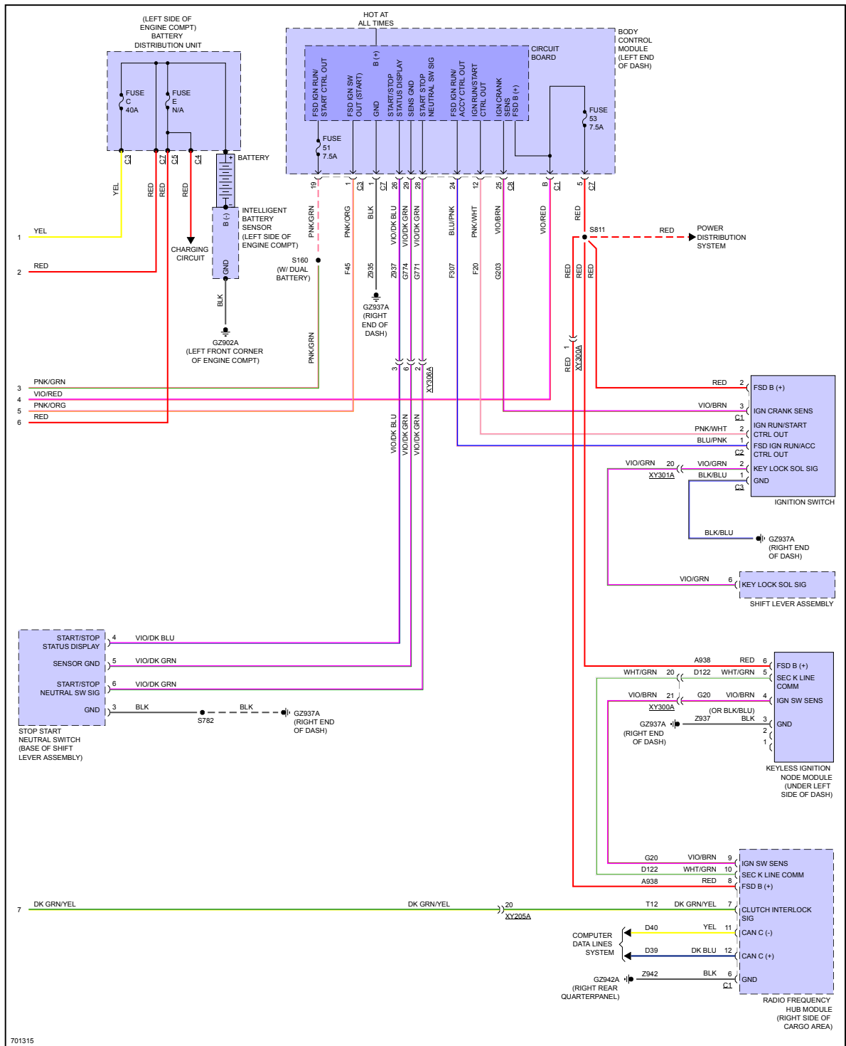
Fig 3: Starting Circuit (2 of 2)
