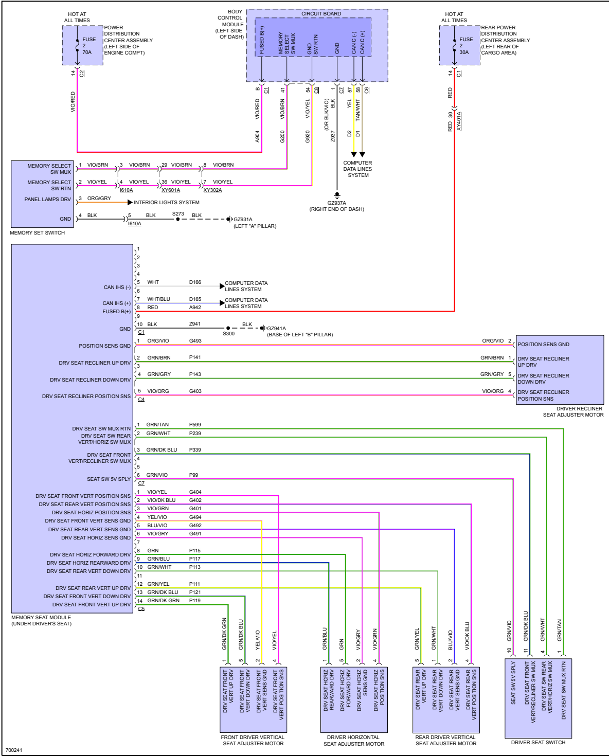
Fig 1: Memory Systems Circuit
