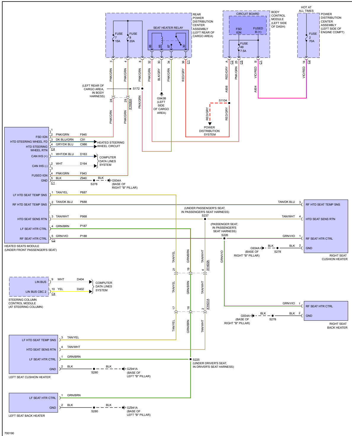
Fig 4: Heated Seats Circuit, W/O Ventilation
