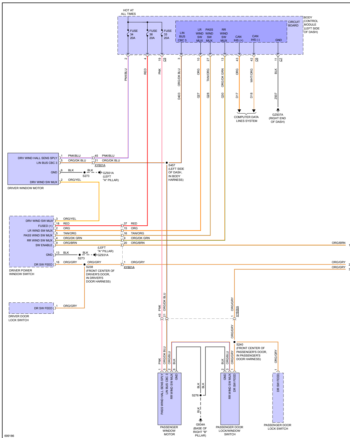
Fig 1: Power Windows Circuit (1 of 2)
