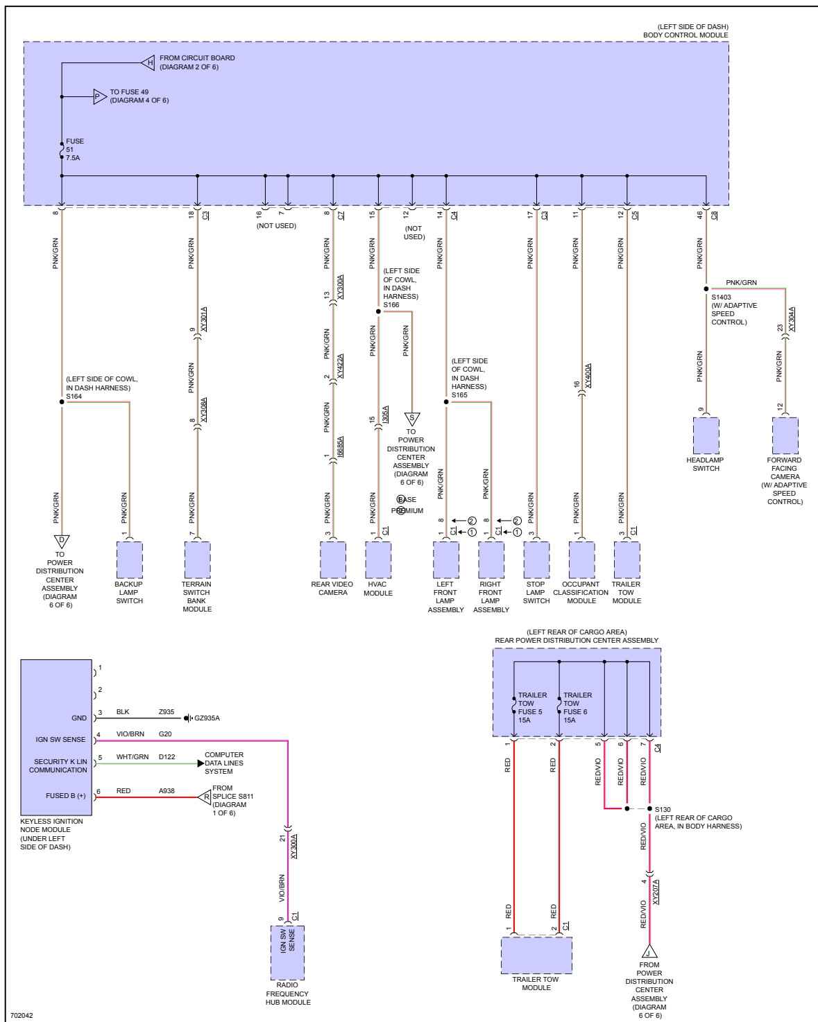
Fig 3: Power Distribution Circuit (3 of 6)
