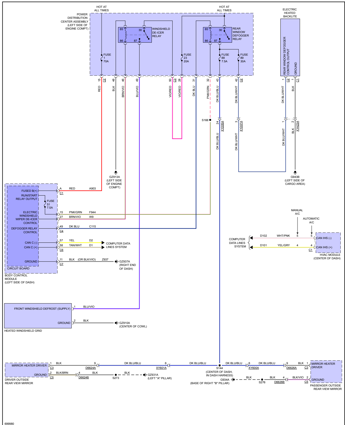
Fig 1: Defoggers Circuit
