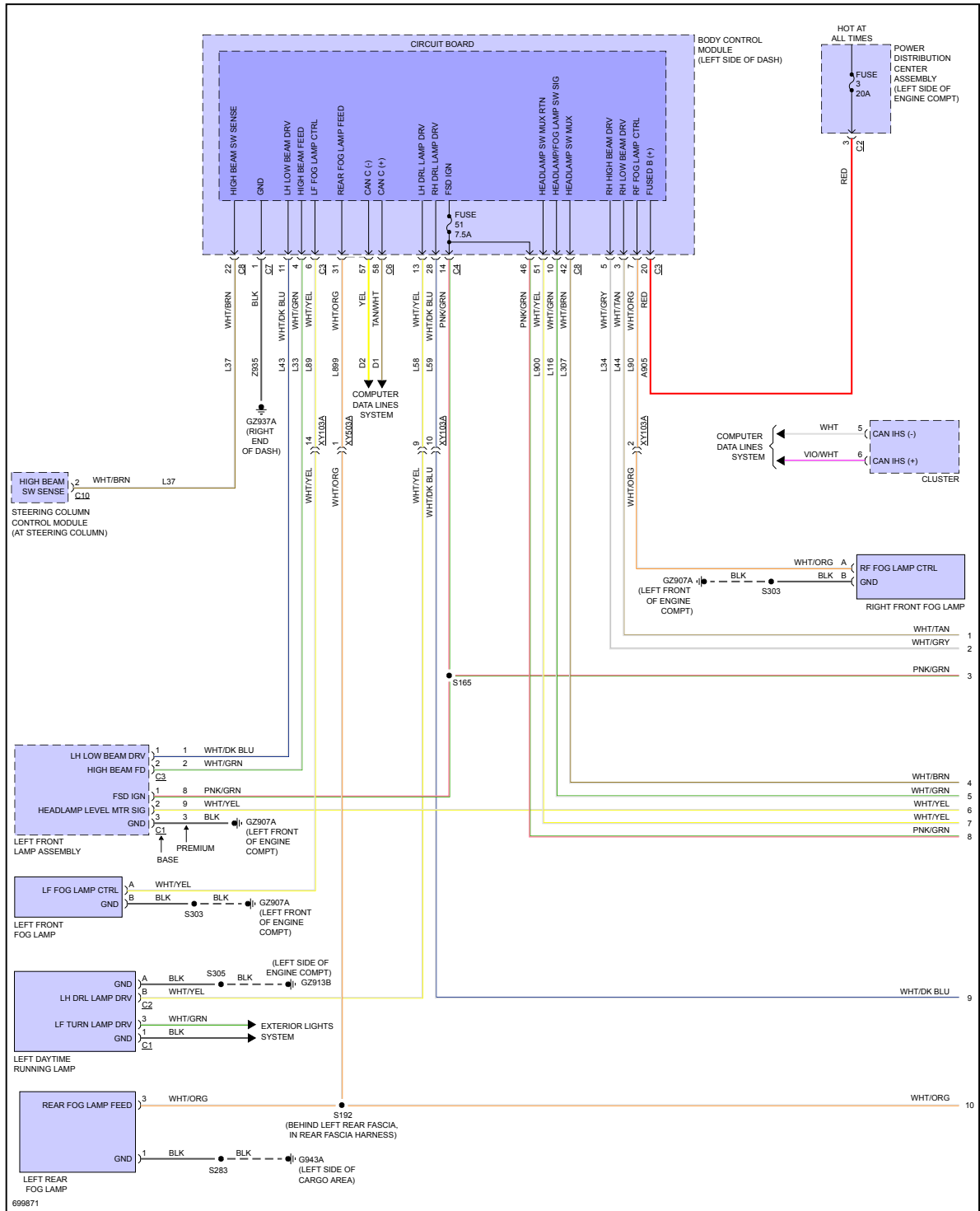
Fig 3: Headlights Circuit, W/O HID (1 of 2)
