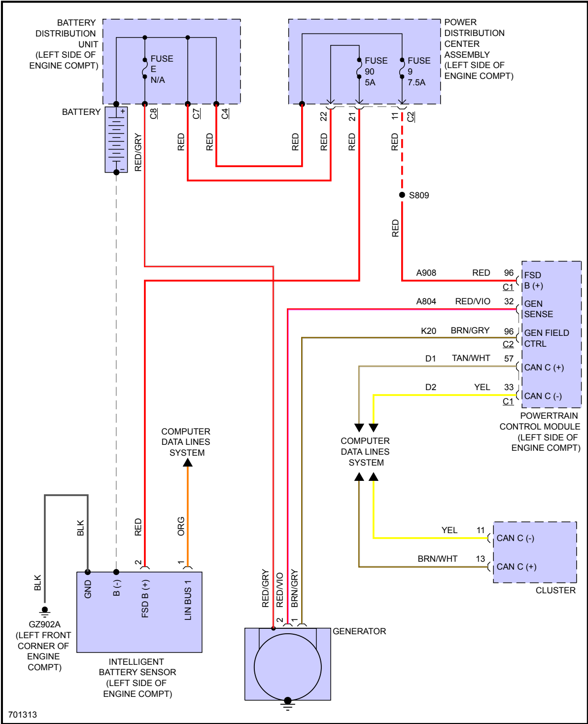
Fig 1: Charging Circuit
