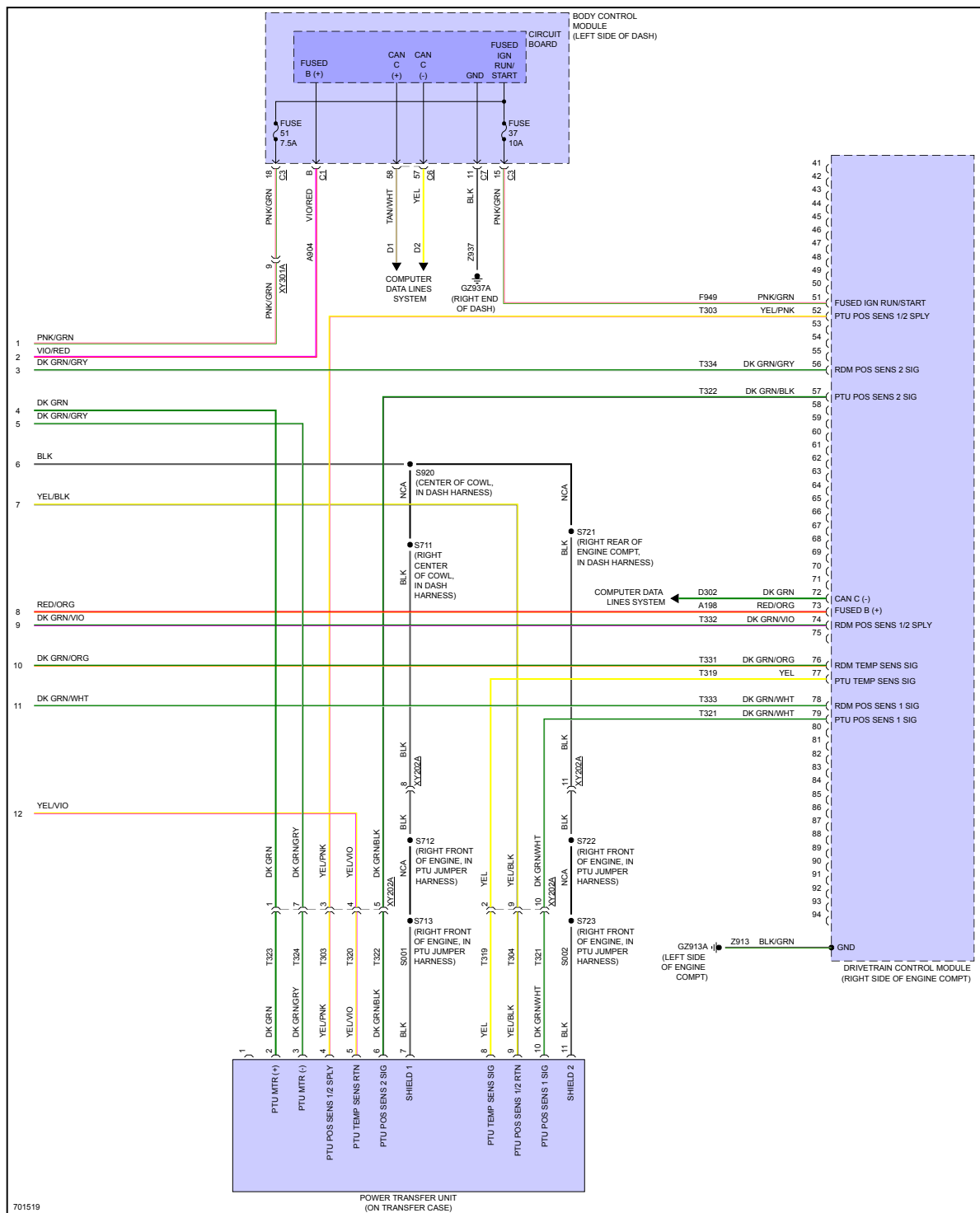
Fig 5: Transfer Case Circuit (2 of 2)
