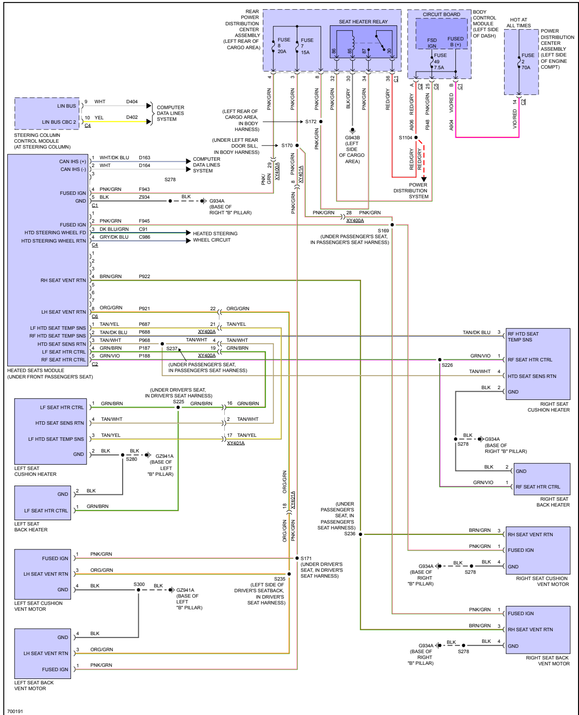
Fig 3: Heated Seats Circuit, W/ Ventilation
