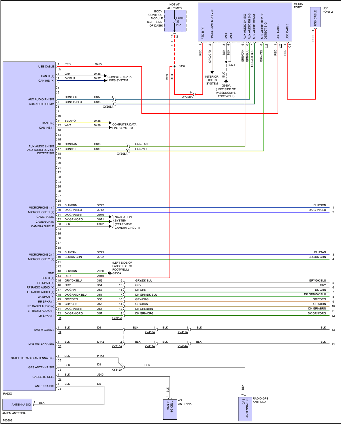
Fig 4: Navigation Circuit, Premium (1 of 3)
