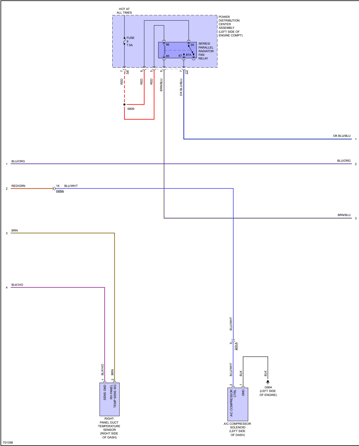
Fig 9: Manual A/C Circuit (4 of 5)
