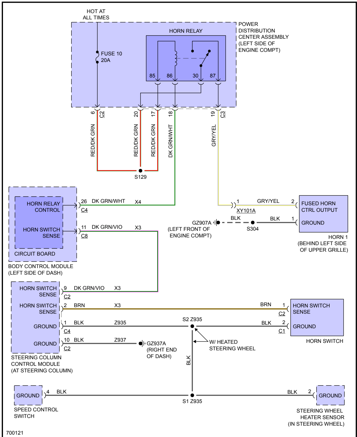
Fig 1: Horn Circuit
