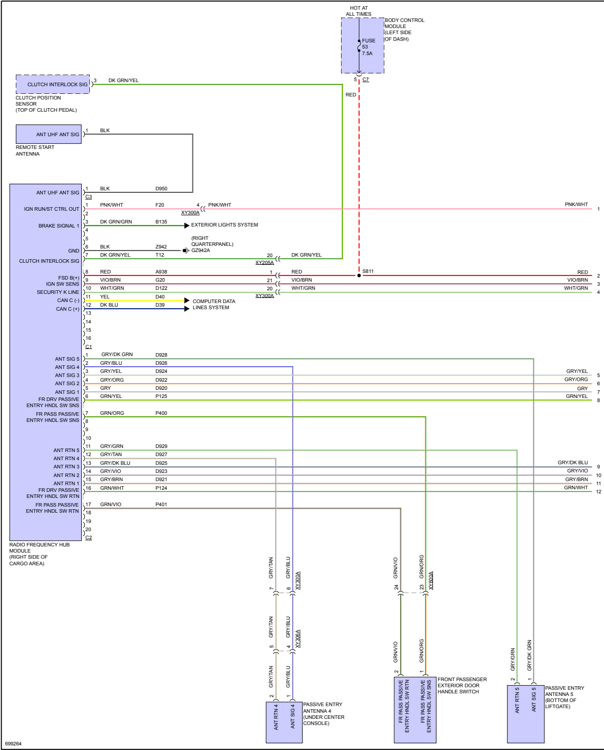
Fig 3: Passive Entry Circuit (1 of 2)
