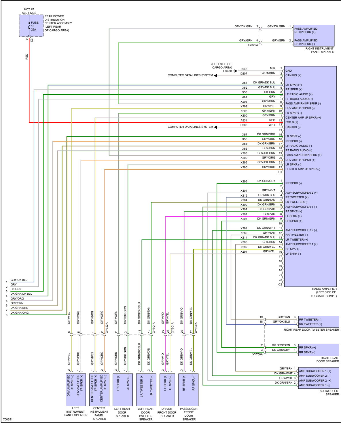
Fig 5: Radio Circuit, Premium (3 of 3)
