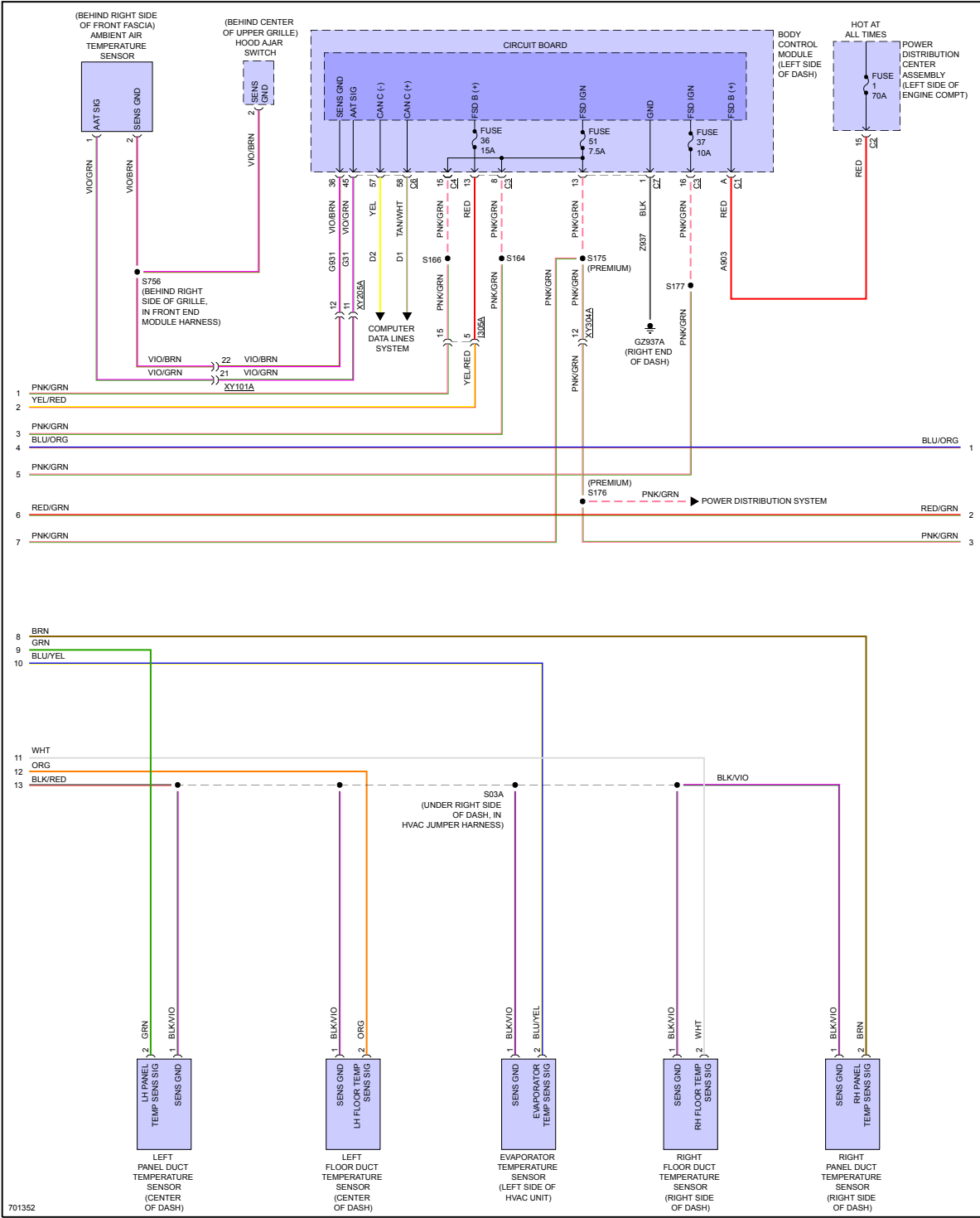
Fig 3: Automatic A/C Circuit (3 of 5)
