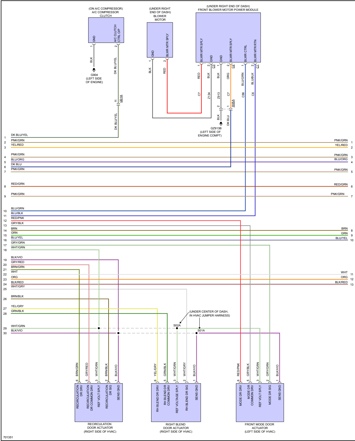
Fig 2: Automatic A/C Circuit (2 of 5)
