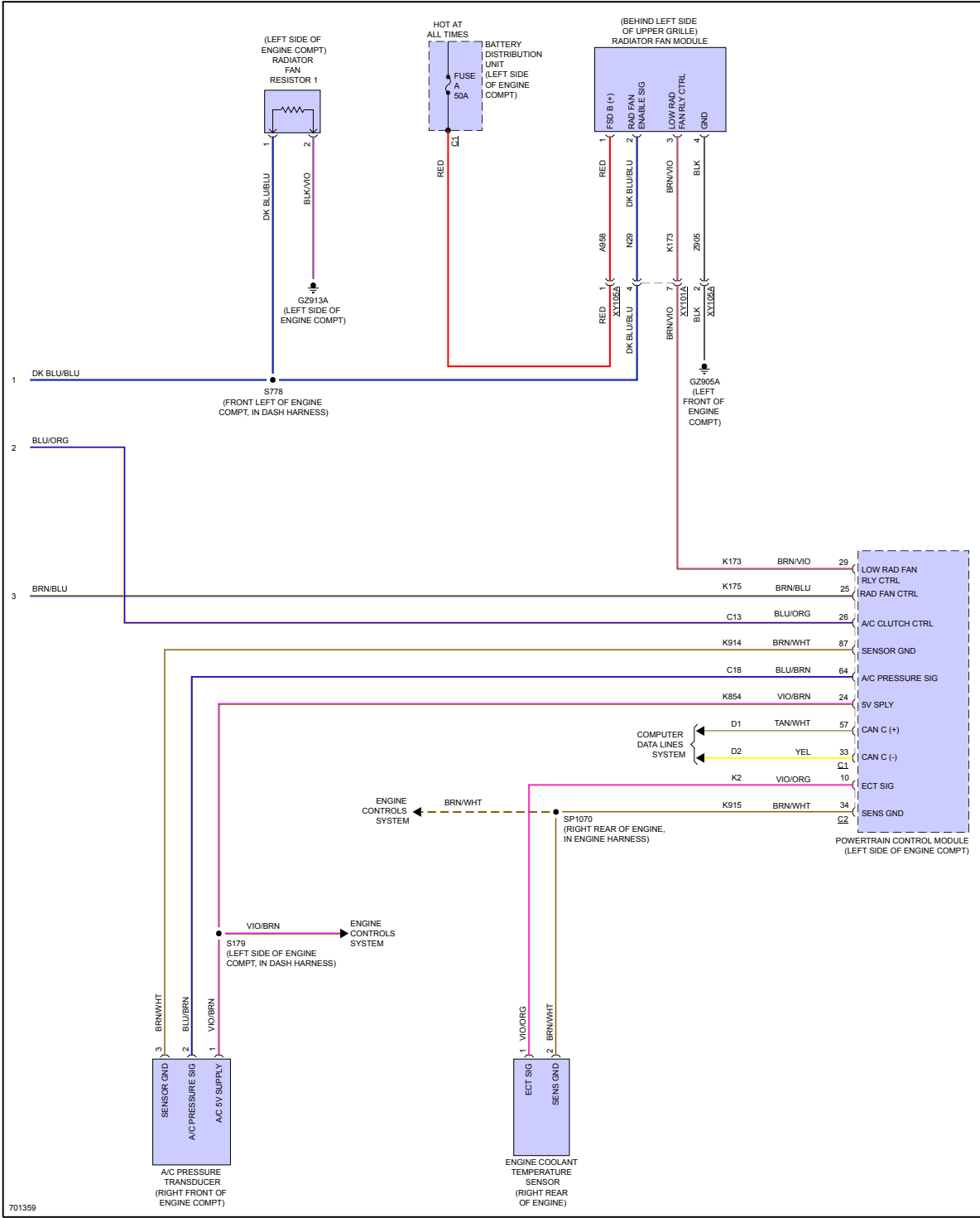
Fig 10: Manual A/C Circuit (5 of 5)
