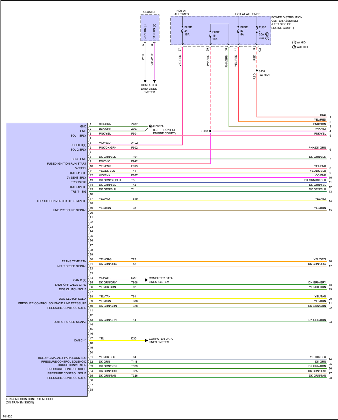
Fig 2: A/T Circuit, 9 Speed A/T (1 of 2)
