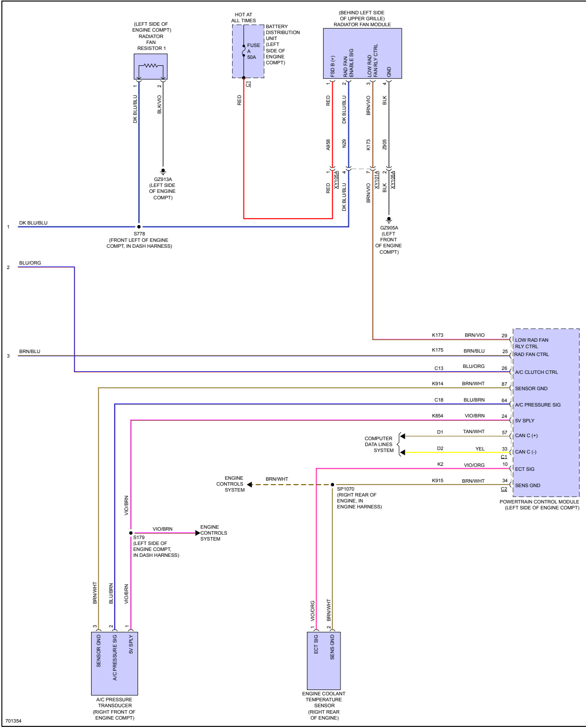
Fig 5: Automatic A/C Circuit (5 of 5)
