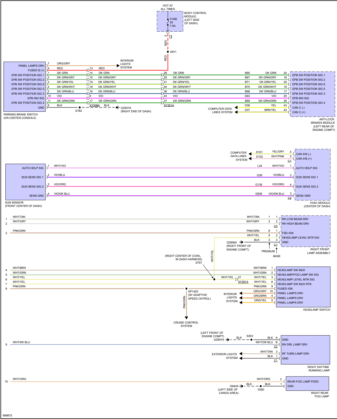
Fig 4: Headlights Circuit, W/O HID (2 of 2)
