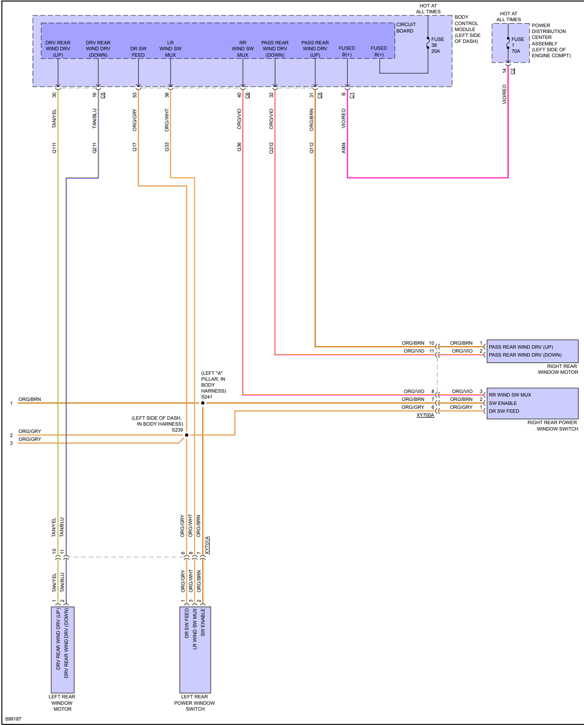
Fig 2: Power Windows Circuit (2 of 2)
