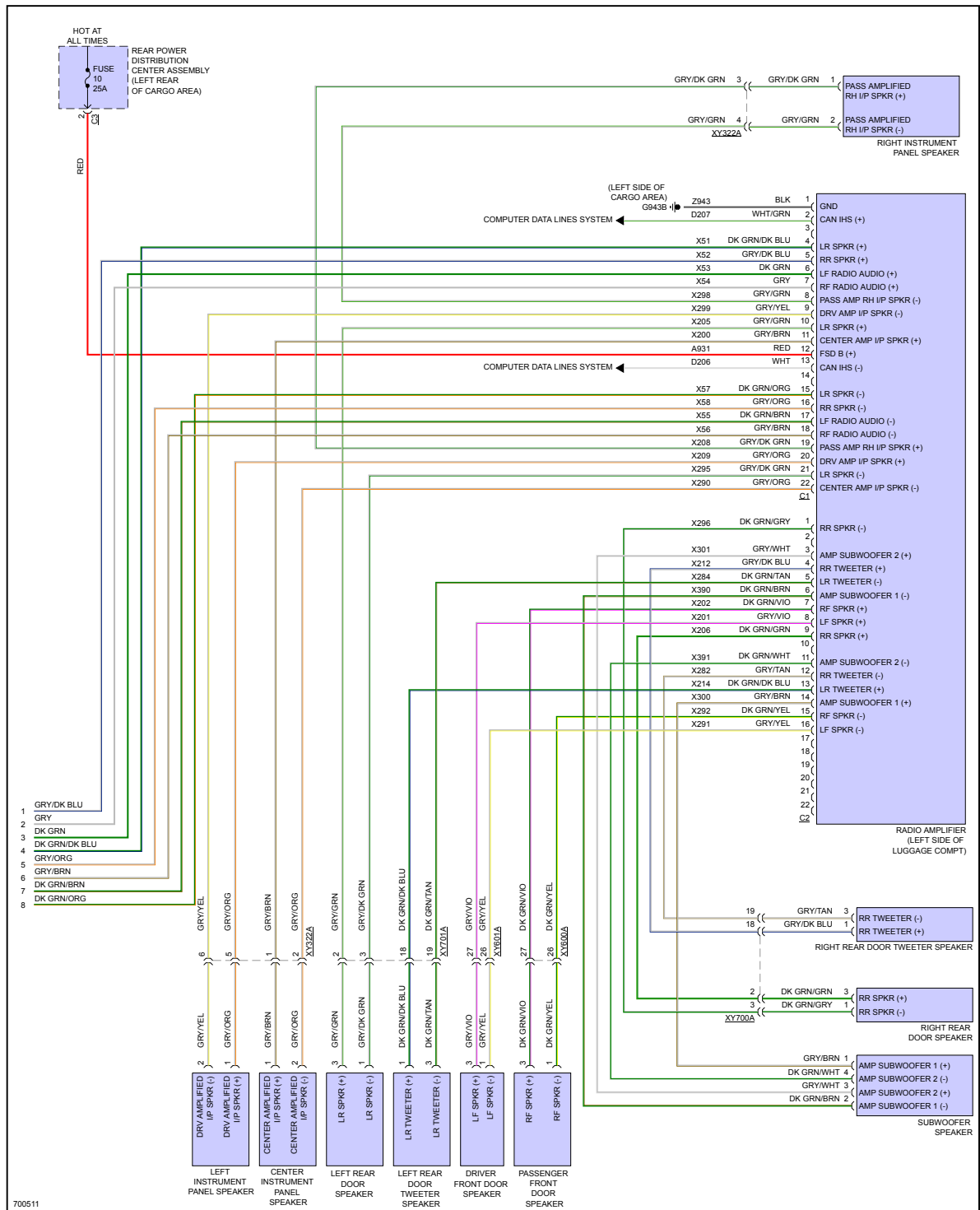
Fig 6: Navigation Circuit, Premium (3 of 3)
