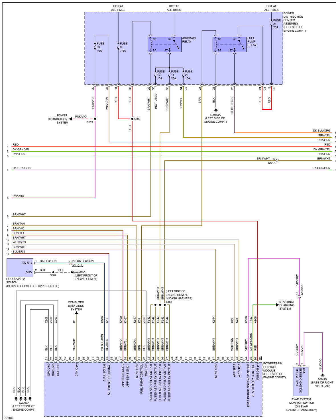
Fig 2: 2.4L, Engine Performance Circuit (2 of 6)
