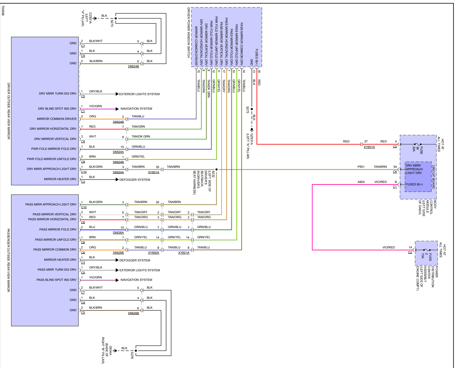
Fig 2: Power Mirrors Circuit
