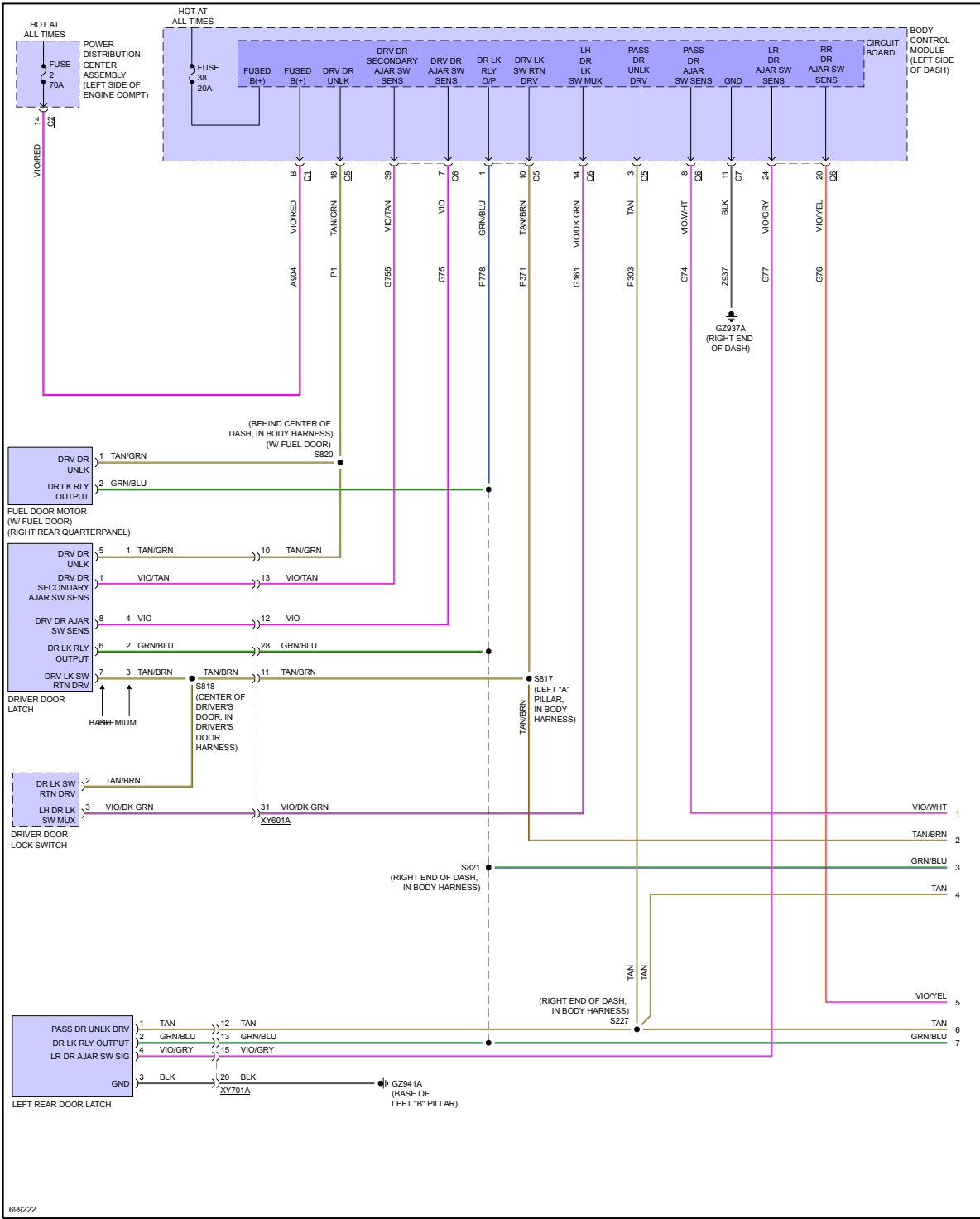
Fig 1: Power Door Locks Circuit (1 of 2)
