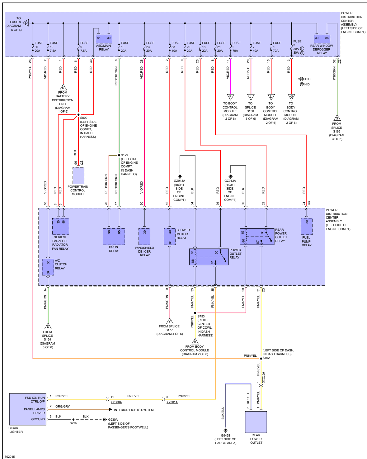
Fig 6: Power Distribution Circuit (6 of 6)
