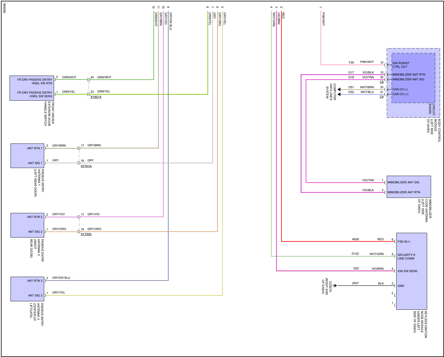
Fig 4: Passive Entry Circuit (2 of 2)
