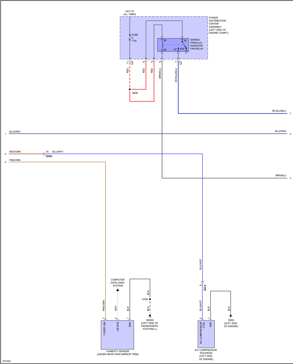
Fig 4: Automatic A/C Circuit (4 of 5)
