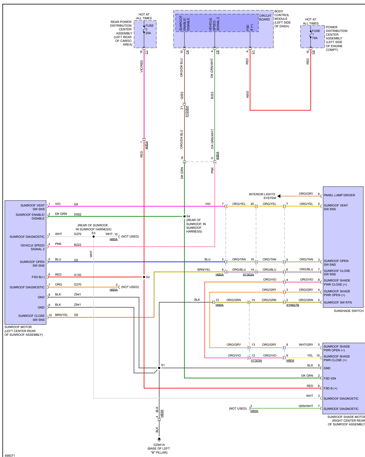
Fig 1: Power Top/Sunroof Circuit
