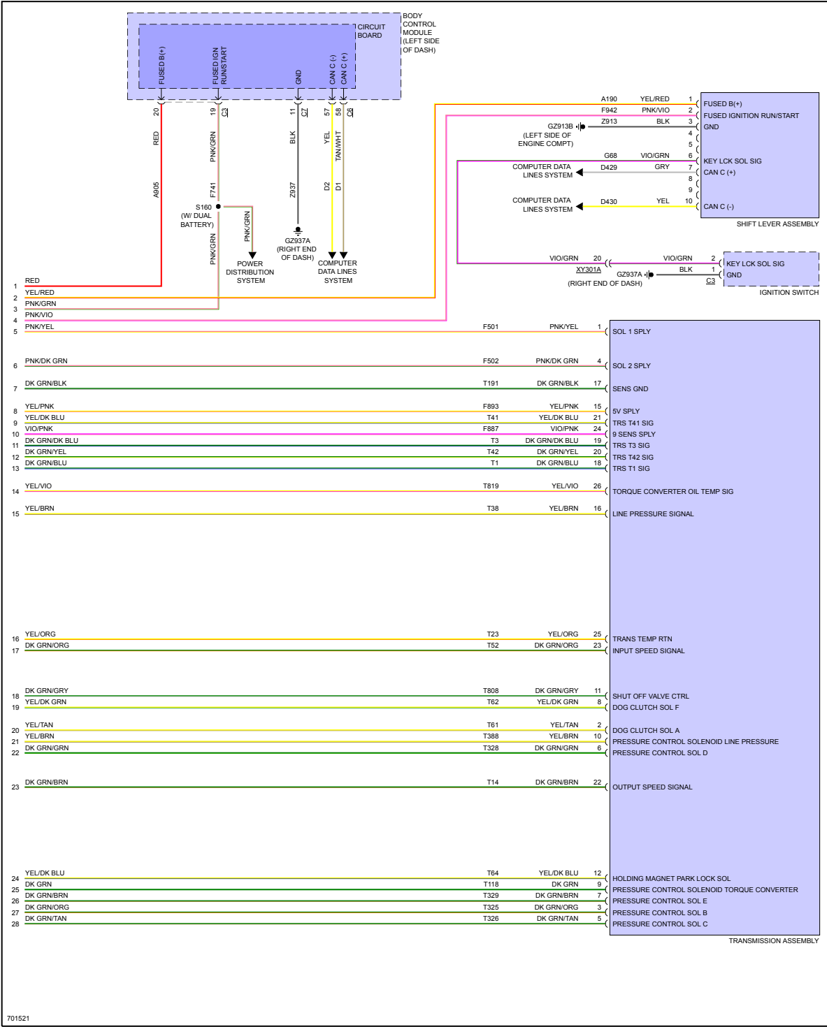
Fig 3: A/T Circuit, 9 Speed A/T (2 of 2)
