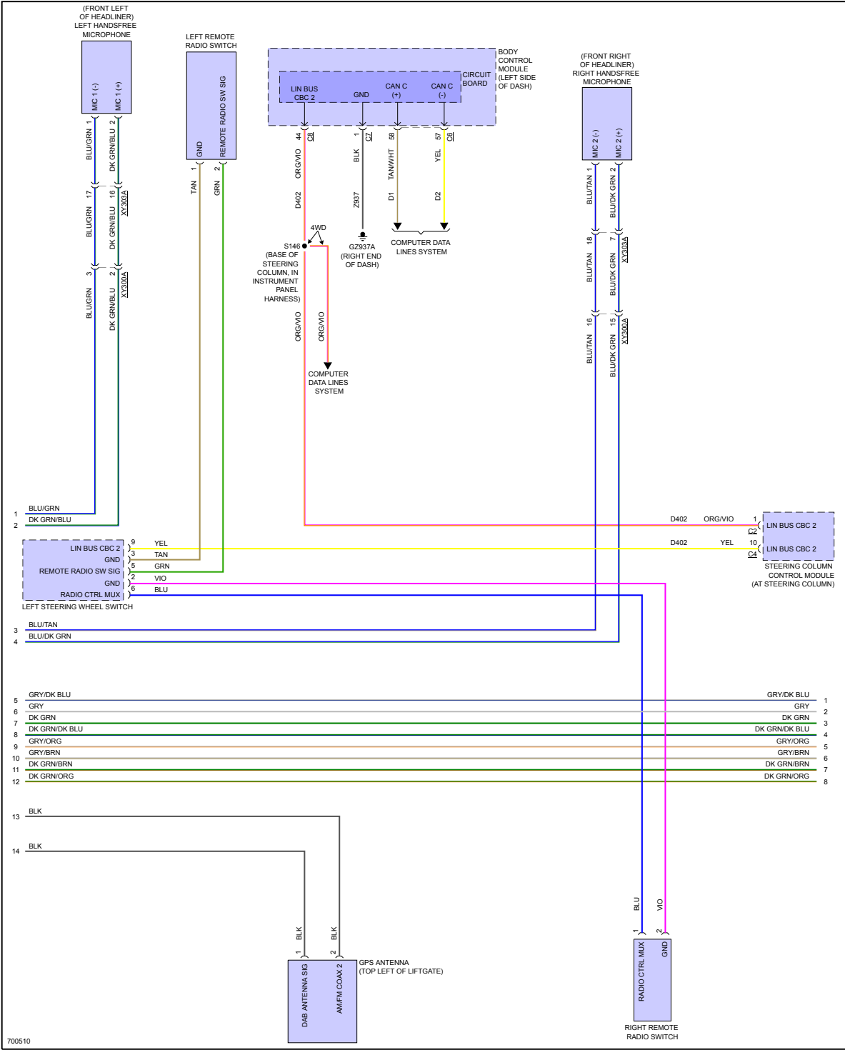
Fig 5: Navigation Circuit, Premium (2 of 3)
