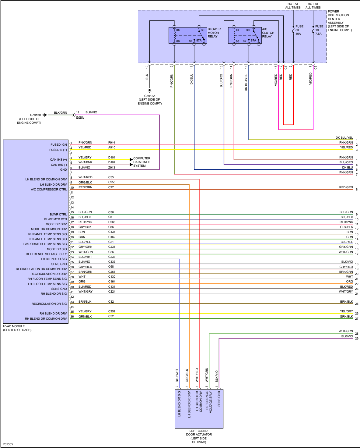
Fig 6: Manual A/C Circuit (1 of 5)
