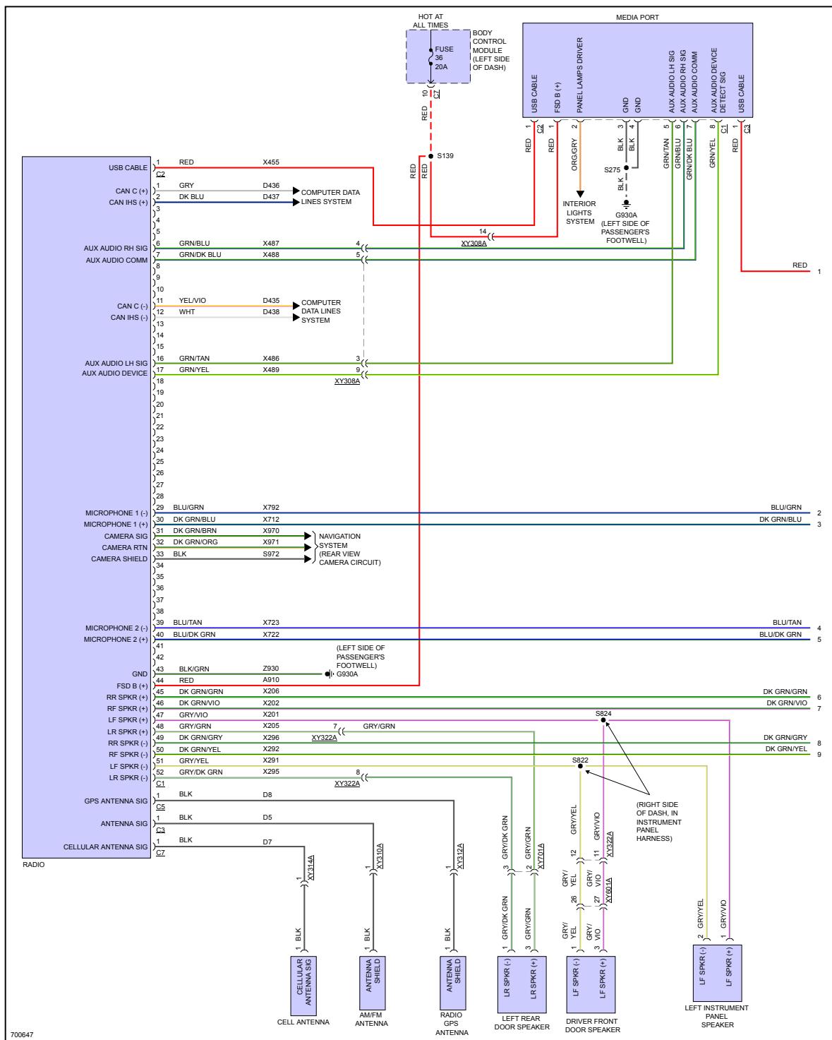
Fig 1: Radio Circuit, Base (1 of 2)
