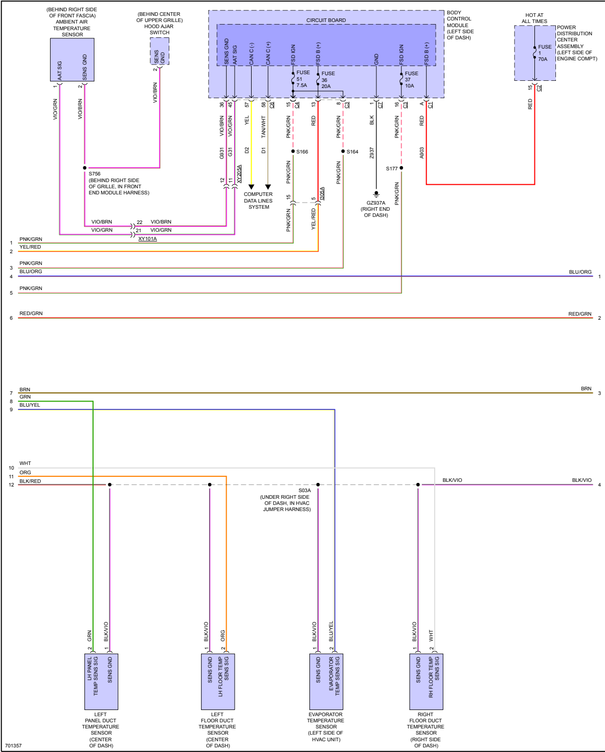
Fig 8: Manual A/C Circuit (3 of 5)
