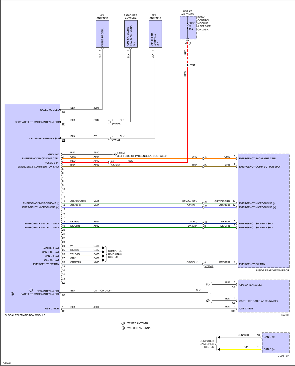
Fig 9: Telematics Circuit
