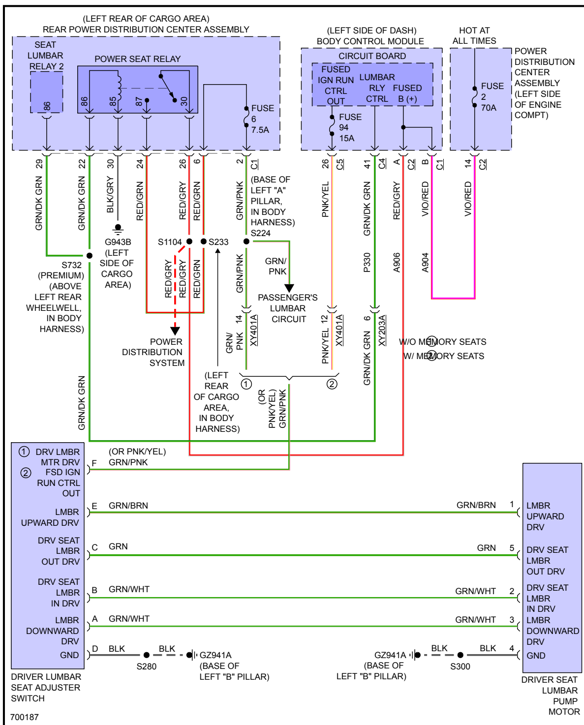
Fig 2: Driver"s Lumbar Circuit
