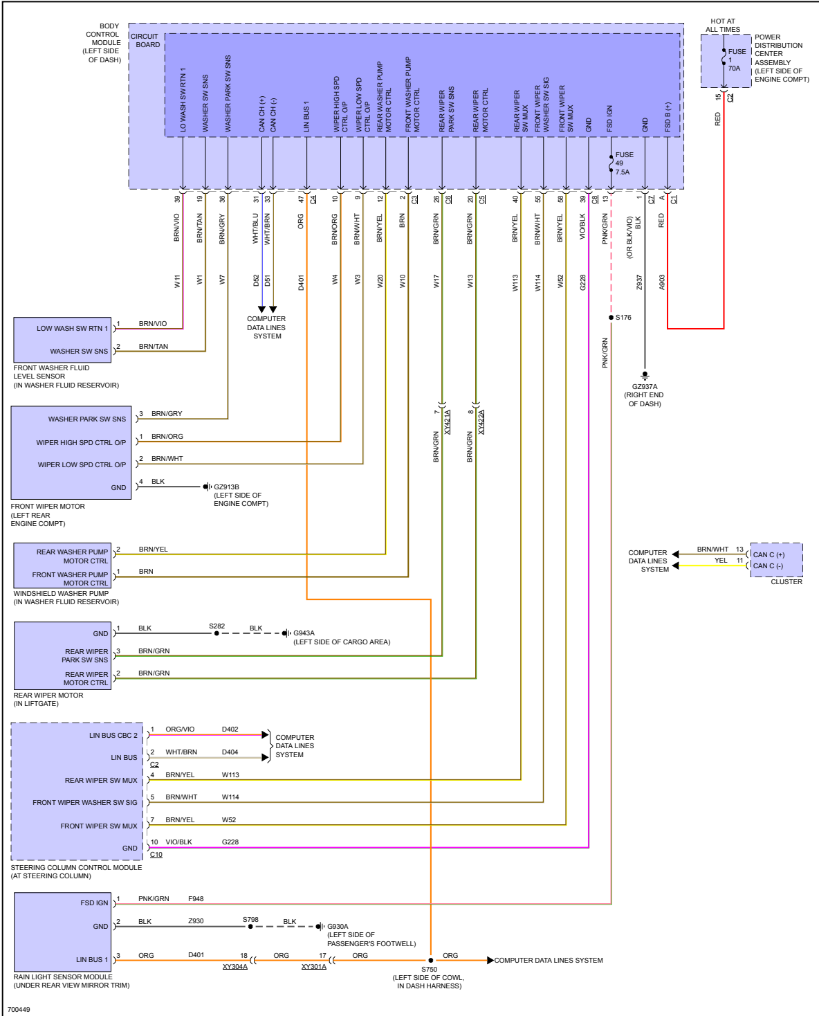
Fig 1: Wiper/Washer Circuit
