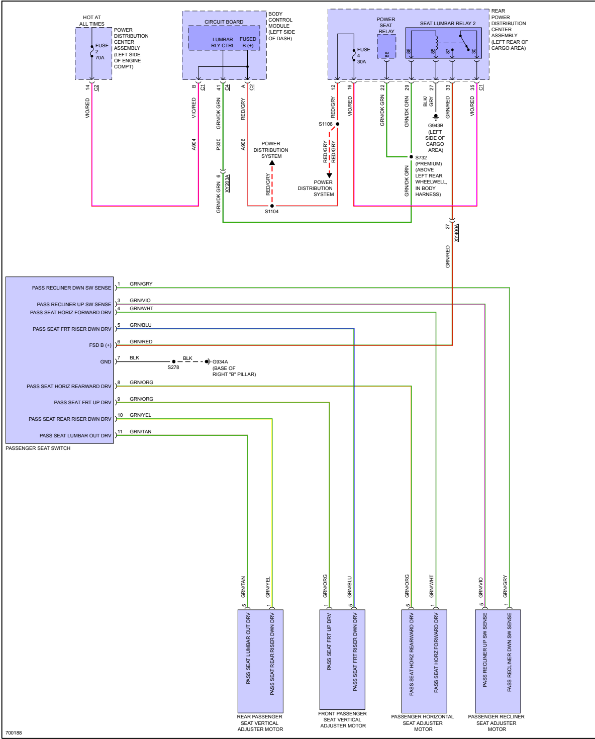
Fig 6: Passenger Power Seat Circuit
