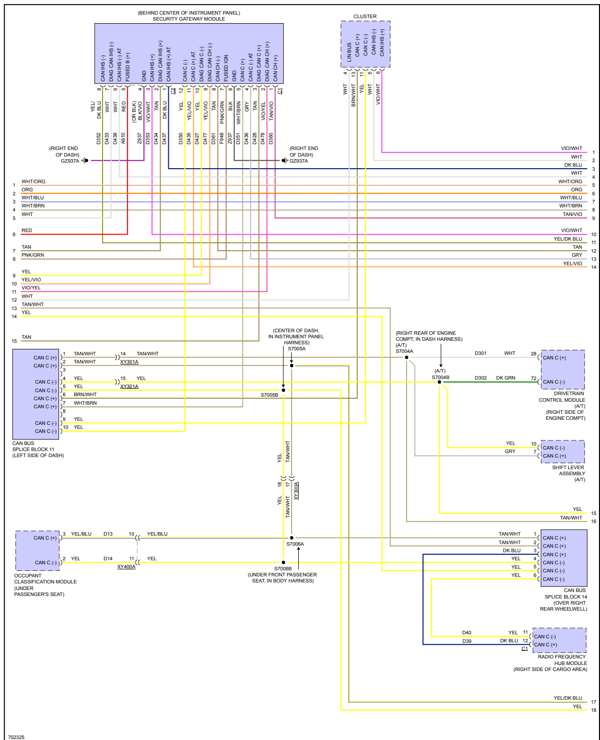
Fig 2: Computer Data Lines Circuit (2 of 5)
