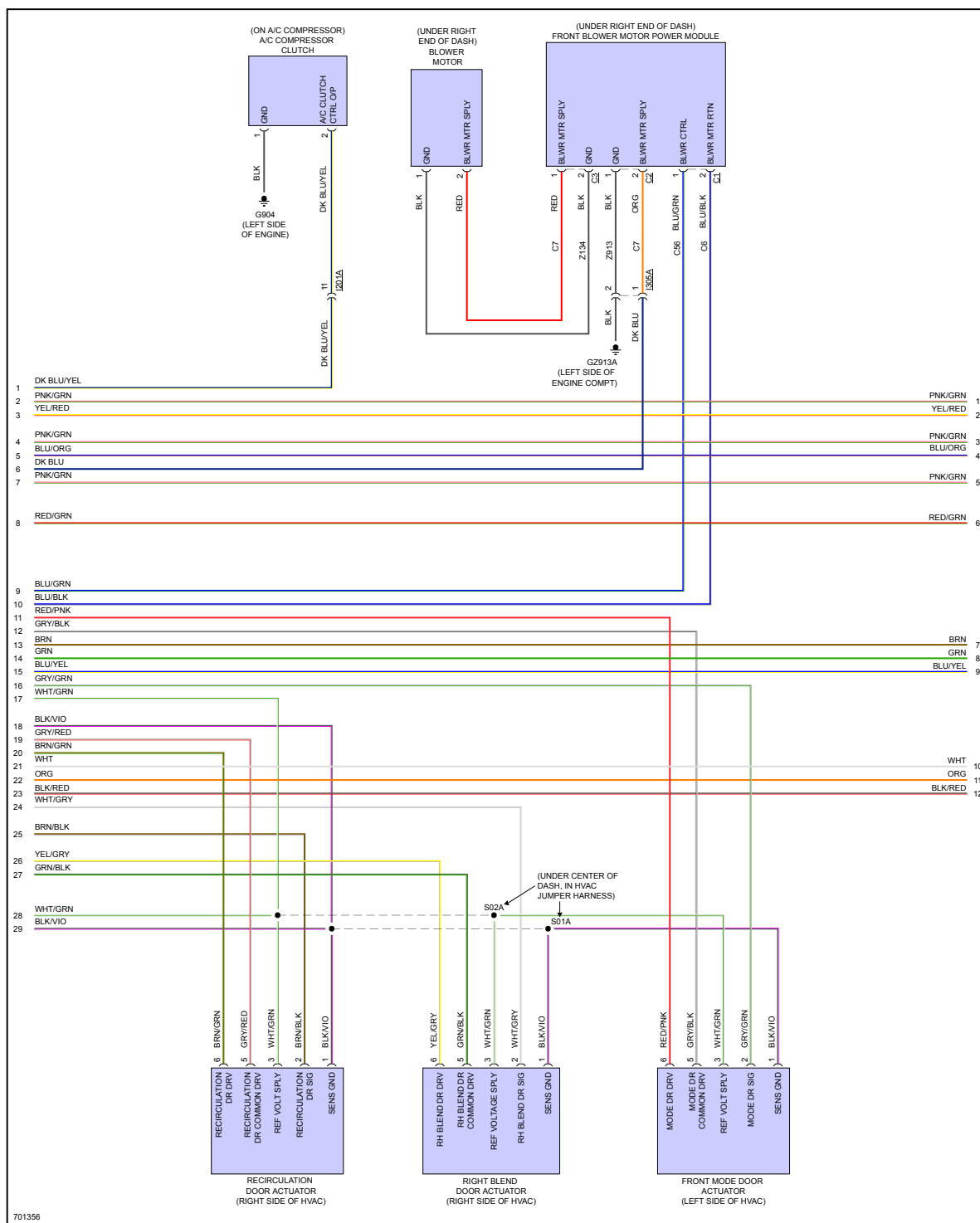
Fig 7: Manual A/C Circuit (2 of 5)
