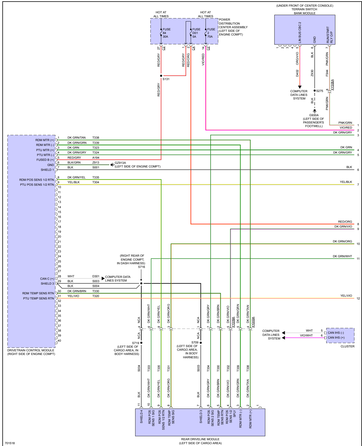
Fig 4: Transfer Case Circuit (1 of 2)
