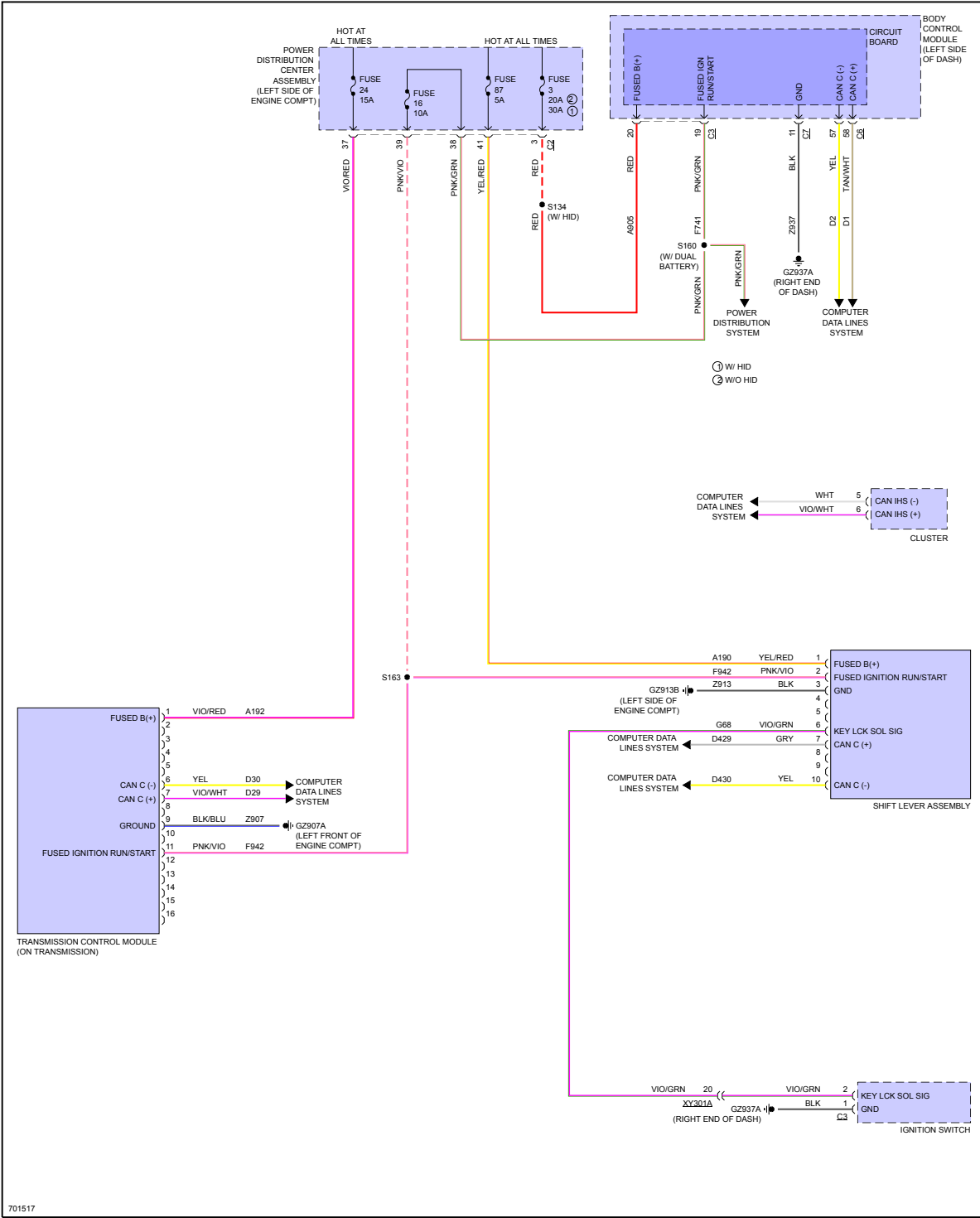
Fig 1: A/T Circuit, 6 Speed A/T
