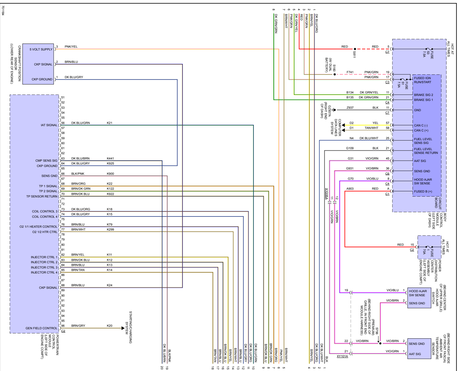
Fig 3: 2.4L, Engine Performance Circuit (3 of 6)
