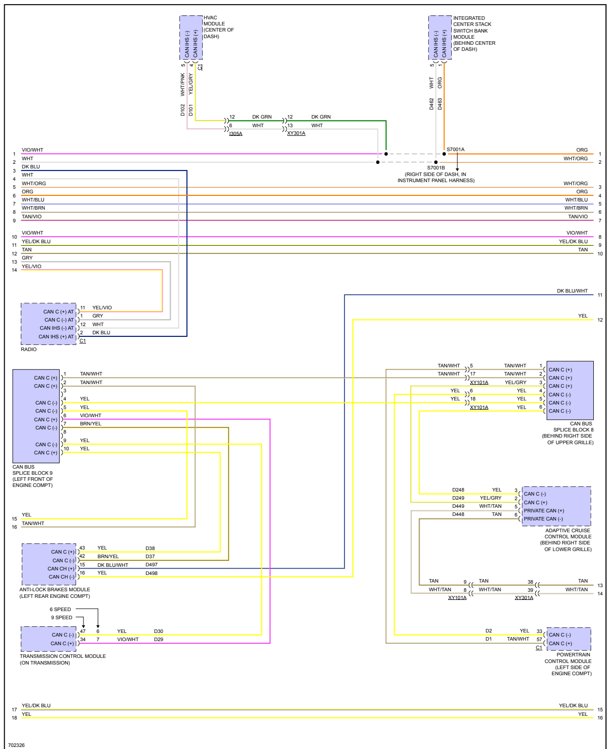
Fig 3: Computer Data Lines Circuit (3 of 5)
