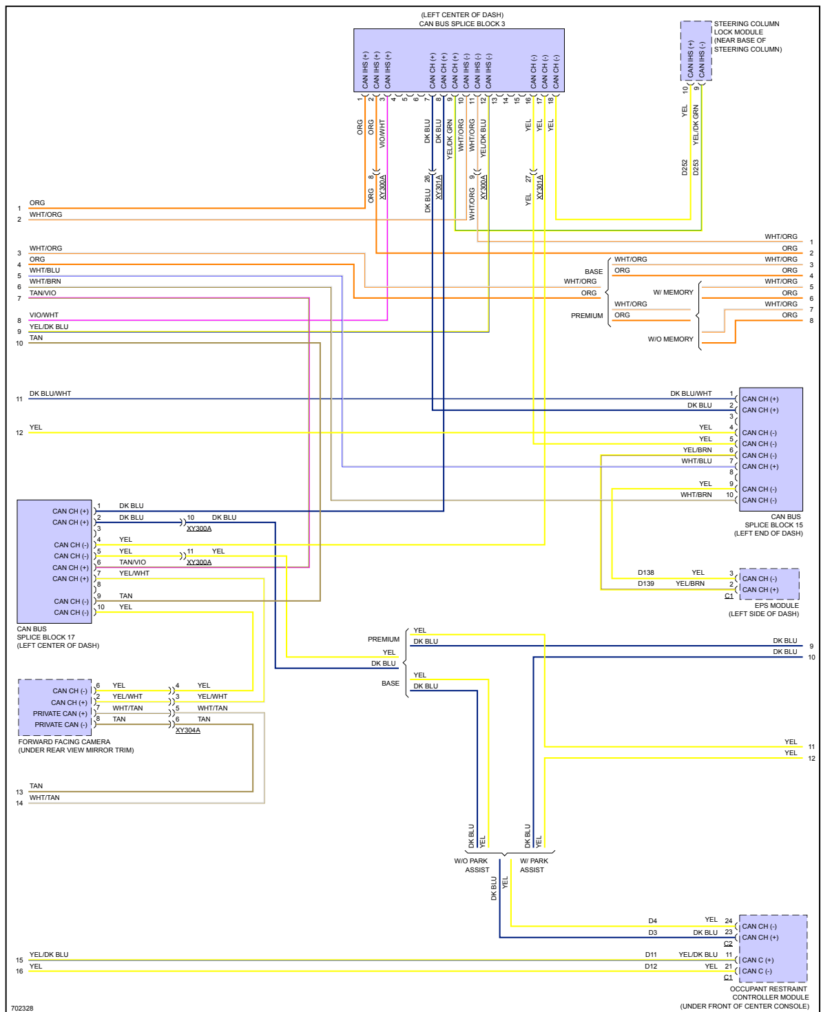
Fig 4: Computer Data Lines Circuit (4 of 5)
