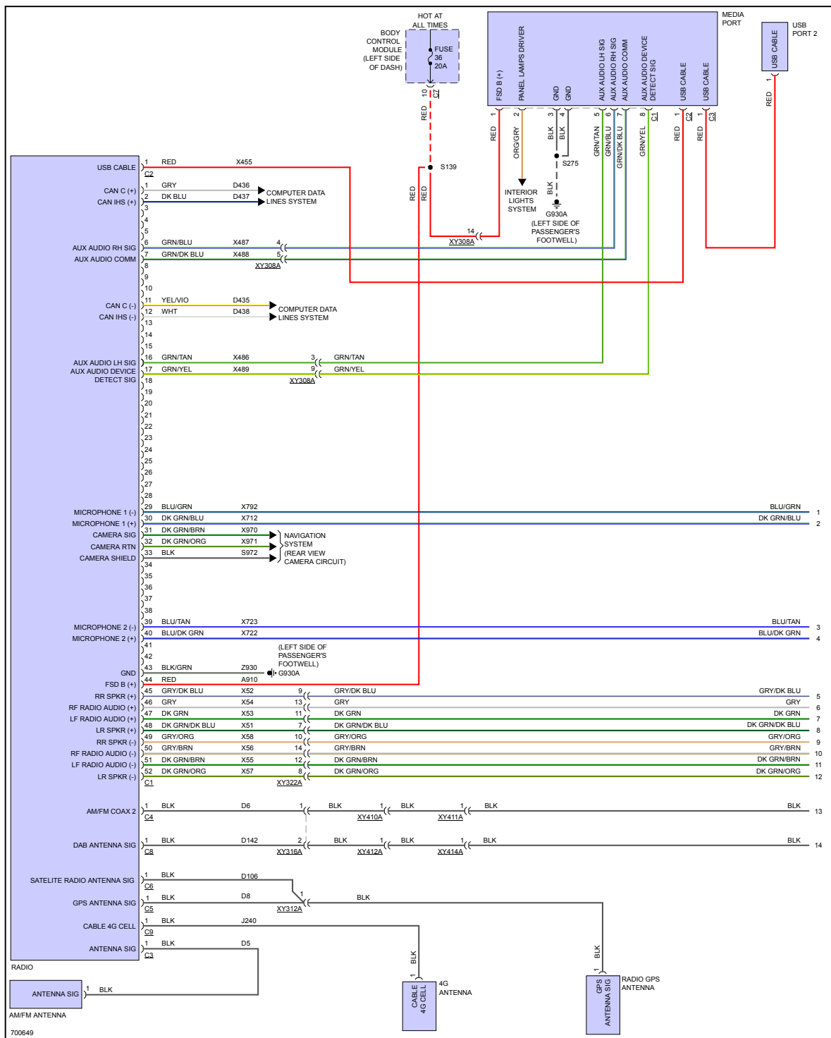
Fig 3: Radio Circuit, Premium (1 of 3)
