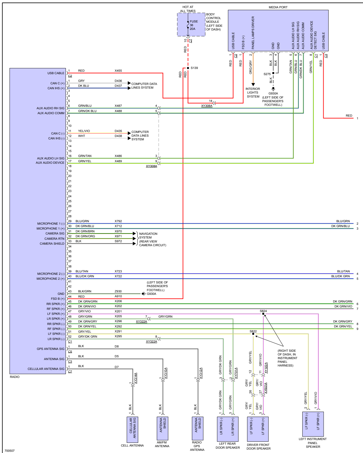
Fig 2: Navigation Circuit, Base (1 of 2)
