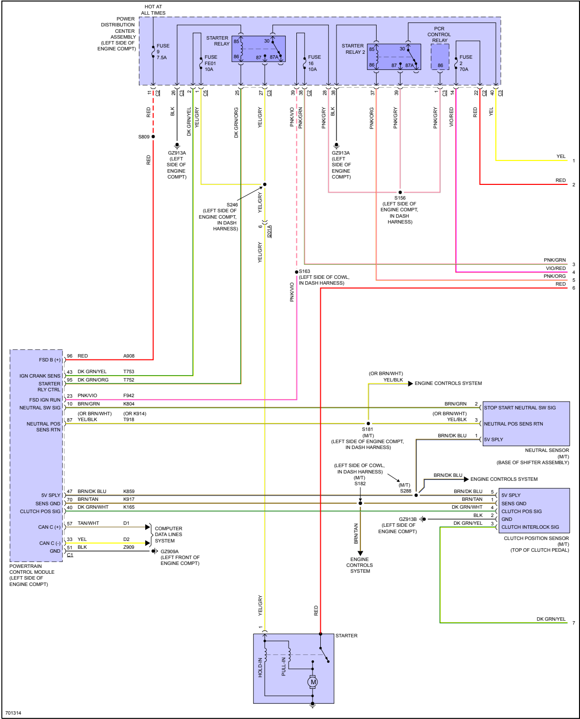
Fig 2: Starting Circuit (1 of 2)
