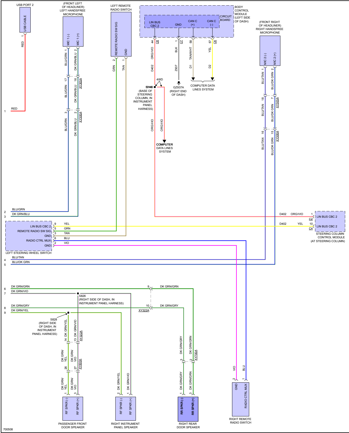
Fig 3: Navigation Circuit, Base (2 of 2)
