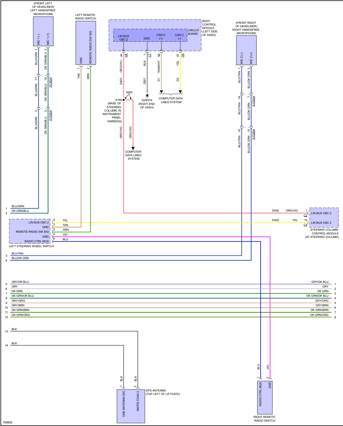
Fig 4: Radio Circuit, Premium (2 of 3)
