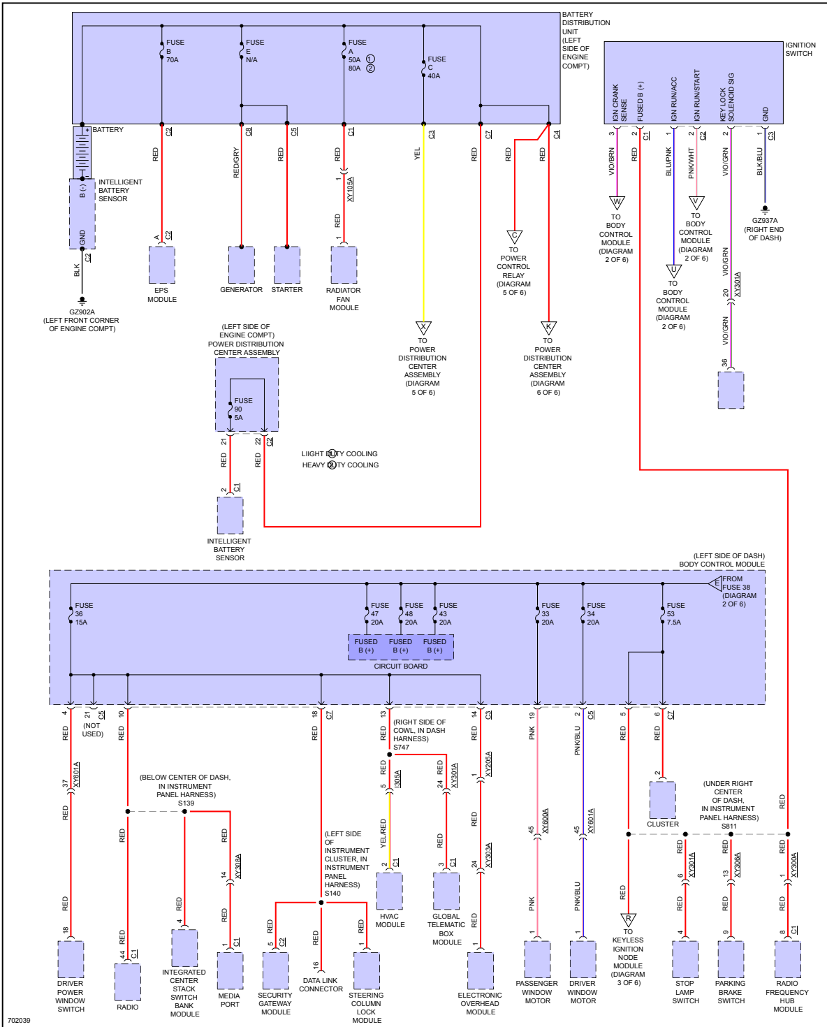
Fig 1: Power Distribution Circuit (1 of 6)
