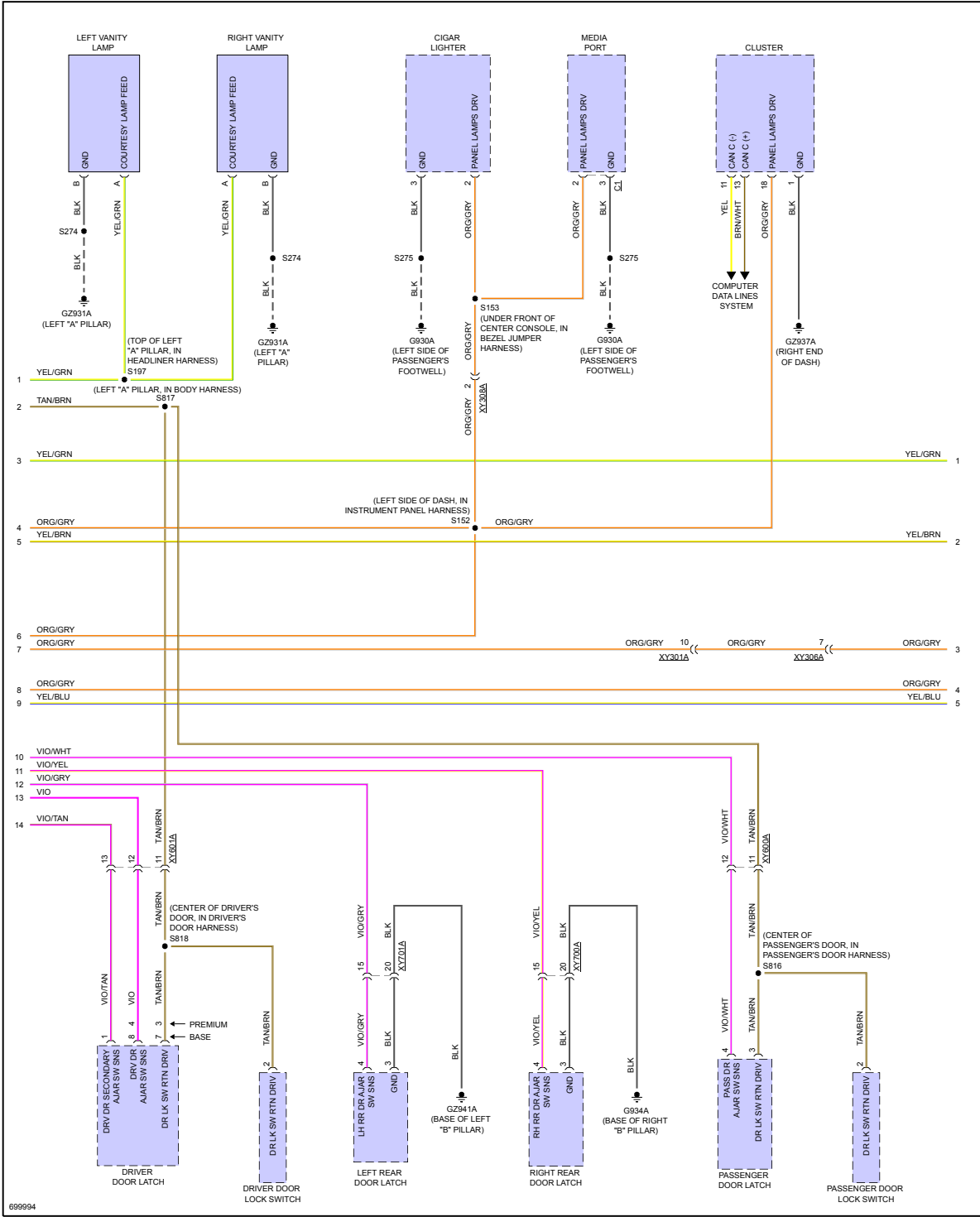
Fig 2: Interior Lights Circuit (2 of 3)
