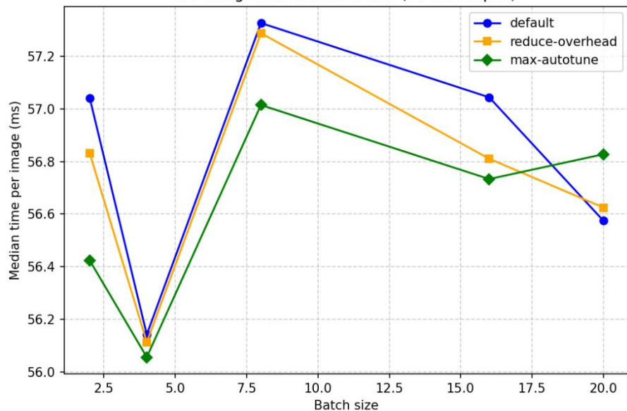
Per-image time vs batch size (torch.compile)
