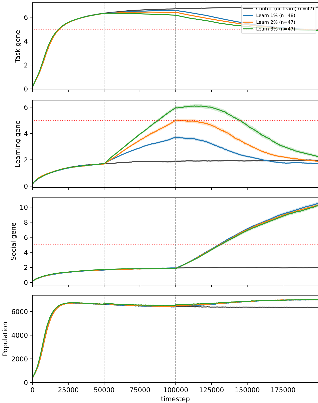
s = 7: mean \pm bootstrap 95% CI
