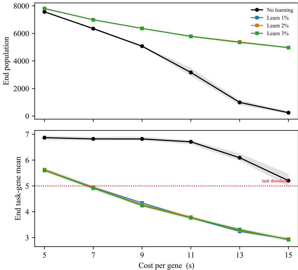
Genetic viability collapses across \approx 10 ; learning rescues it
