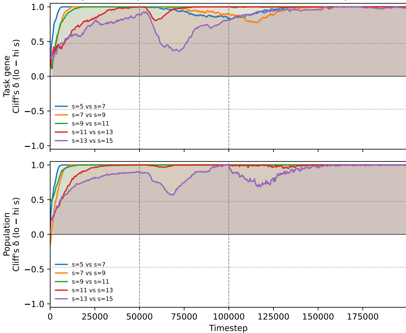
Adjacent-s separation over time (learn 2%); shaded = p < 0.05
