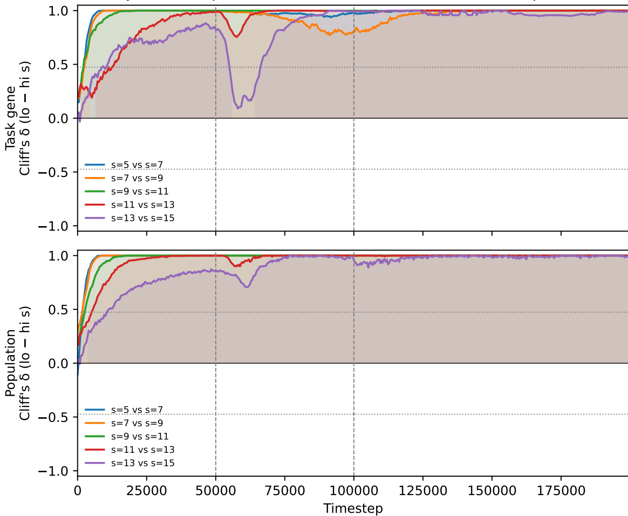
Adjacent-s separation over time (learn 3%); shaded = p < 0.05
