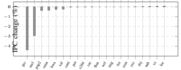
Fig. 5. Per-program IPC change, gated stride vs. raw stride (sorted). Only GCC (−4.4%) and MCF (−2.9%) are outliers; the remaining 18 programs fall within \pm 0.4\% .
