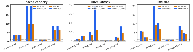
Fig. 7. Machine sensitivity: NN vs. stride speedup for two settings of cache capacity, DRAM latency, and line size. The NN’s safety on random persists across all settings.
