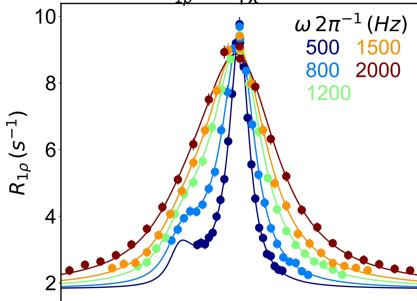
R_{1\rho} Plot | \bar{\chi}^2 0.99
