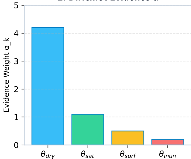
1. Dirichlet Evidence \alpha
