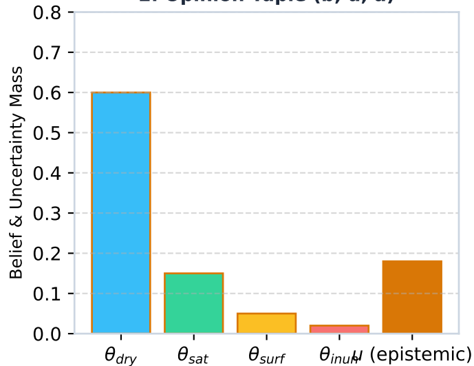
2. Opinion Tuple (b, u, a)
