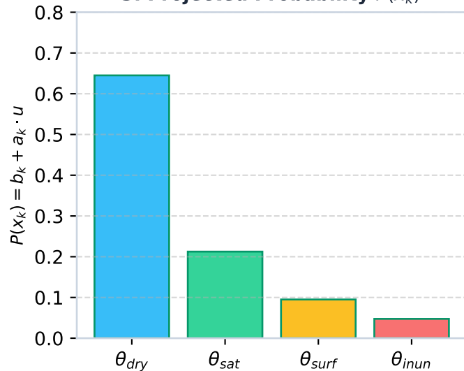
3. Projected Probability P(x_k)
