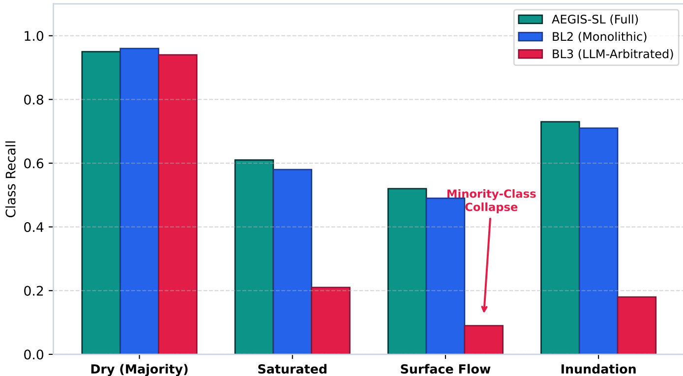
Per-Class Recall & LLM Minority-Class Collapse Diagnostic ($6.3 H2)
