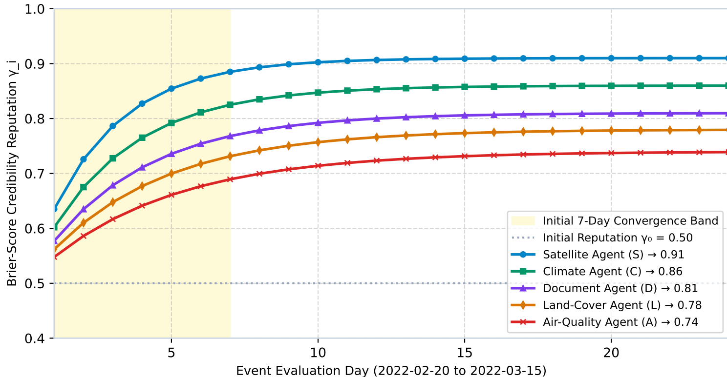
24-Day Per-Agent Credibility Trajectory & Online Convergence ($6.5 H4)
