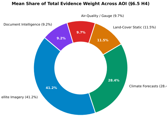
Figure 9: Mean Share of Total Evidence Weight Across AOI (H4 Part 2). Relative evidence contribution across the 24-day evaluation window: Satellite Imagery (41.2%), Climate Forecasts (28.4%), Land-Cover (11.5%), Air-Quality/Gauge (9.7%), and Document Intelligence (9.2%).
