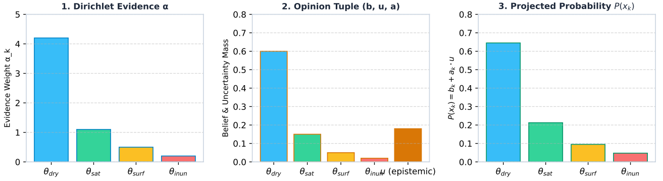
Figure 1: Subjective Logic Opinion Mapping & Partial Projection Pipeline. Bijective transformation from Dirichlet evidence parameters \alpha = (\alpha_1, \alpha_2, \alpha_3, \alpha_4) onto opinion tuple \omega = (\mathbf{b}, u, \mathbf{a}) and projected expected probability P(x_k) = b_k + a_k \cdot u . When a modality drops, the partial-observable projection rule ( \alpha_k^{\text{proj}} = C \cdot a_k ) forces belief mass b_k \rightarrow 0 and raises epistemic uncertainty u \rightarrow 1.0 monotonically.
