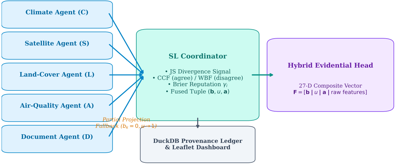
Figure 2: AEGIS System Architecture Flow. Heterogeneous environmental streams map onto five specialist evidential agents (Climate, Satellite, Land-Cover, Air-Quality/Gauge, Document Intelligence). Active opinion streams \omega_i route through the SL Coordinator (with JS divergence signal \tau_{\text{low}} = 0.1 ) to produce fused opinion \mathbf{F} = (\mathbf{b}, u, \mathbf{a}) . The 27-dimensional composite space feeds the Hybrid LightGBM Head while logging provenance to DuckDB and powering the Leaflet dark-mode dashboard.
