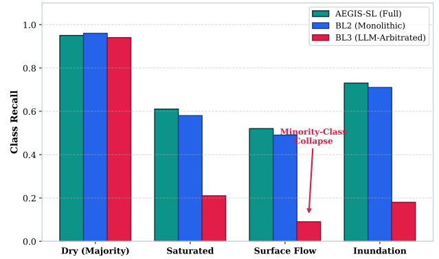
Figure 6: Per-Class Recall & LLM Minority-Class Collapse Diagnostic (H2). Grouped recall comparison across flood classes. Prompt-chained LLM arbitration (BL3) collapses on minority classes (saturated 0.21, surface 0.09, inundation 0.18), whereas AEGIS-SL maintains strong recall across all states.
