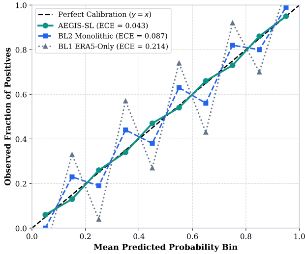
Figure 5: Calibration Reliability Diagram Across Baselines (H1). Bin-wise predicted confidence vs observed positive fraction over 10 equal-width bins. AEGIS-SL (ECE 0.043) closely tracks the ideal y = x diagonal, outperforming monolithic BL2 (ECE 0.087) and ERA5-only BL1 (ECE 0.214).
