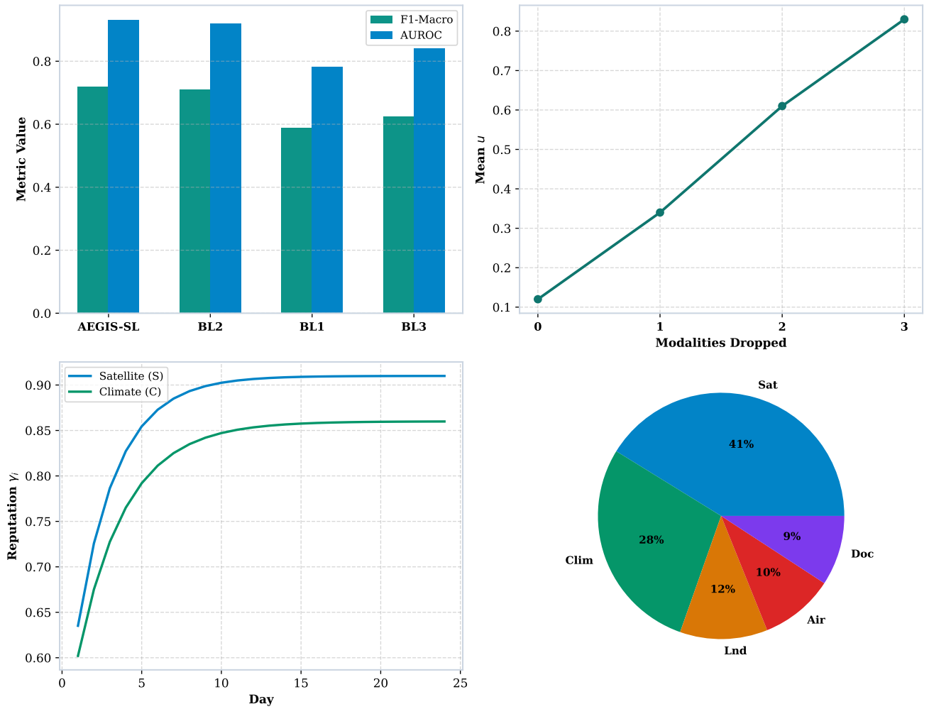
Figure 4: AEGIS Empirical Evaluation Master Composite Panel. 2x2 small-multiple panel summarizing the core empirical findings: (A) Overall accuracy (H1); (B) Monotonic epistemic uncertainty u (H3); (C) Per-agent credibility convergence (H4); and (D) Mean source evidence shares.
