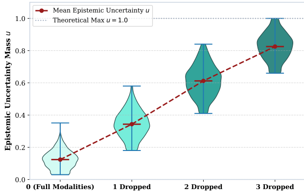
Figure 7: Monotonic Epistemic Uncertainty u Under Sensor Dropout (H3). Distribution of cell-wise u values across 0, 1, 2, and 3 dropped modalities. Mean u (red overlay) rises strictly monotonically ( 0.12 \rightarrow 0.34 \rightarrow 0.61 \rightarrow 0.83 ) without false-confidence subtraction, verifying Theorem 1.
