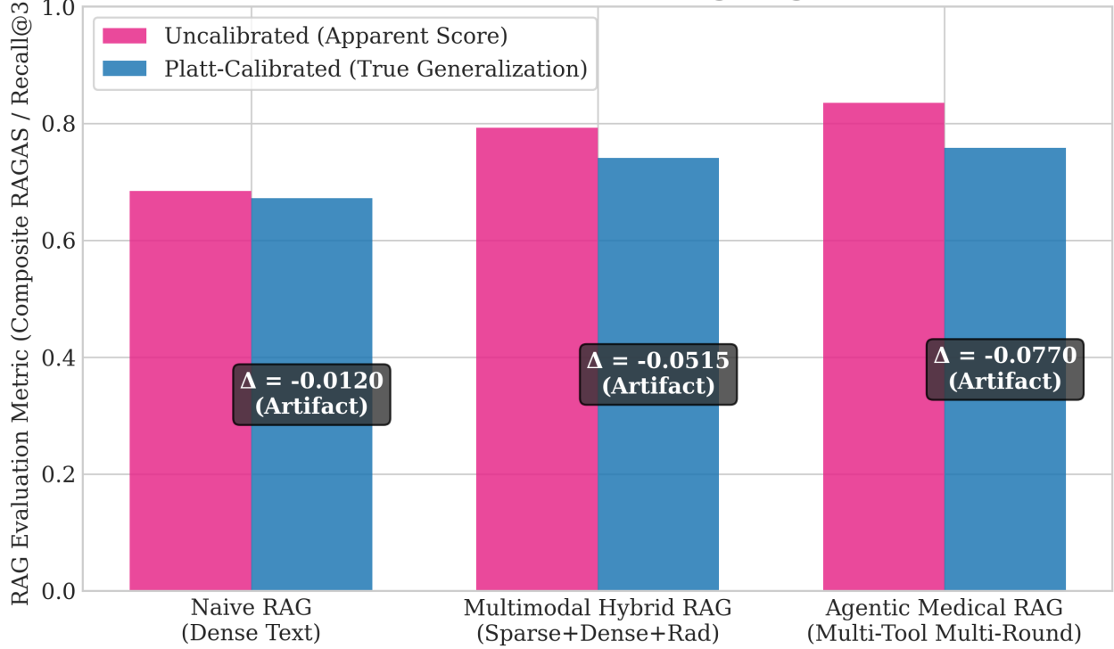
Figure 5: Architectural shrinkage: Uncalibrated vs. Calibrated composite RAGAS scores across Naive, Multimodal Hybrid, and Agentic RAG architectures, demonstrating the dissolution of apparent performance gains under probability calibration.
