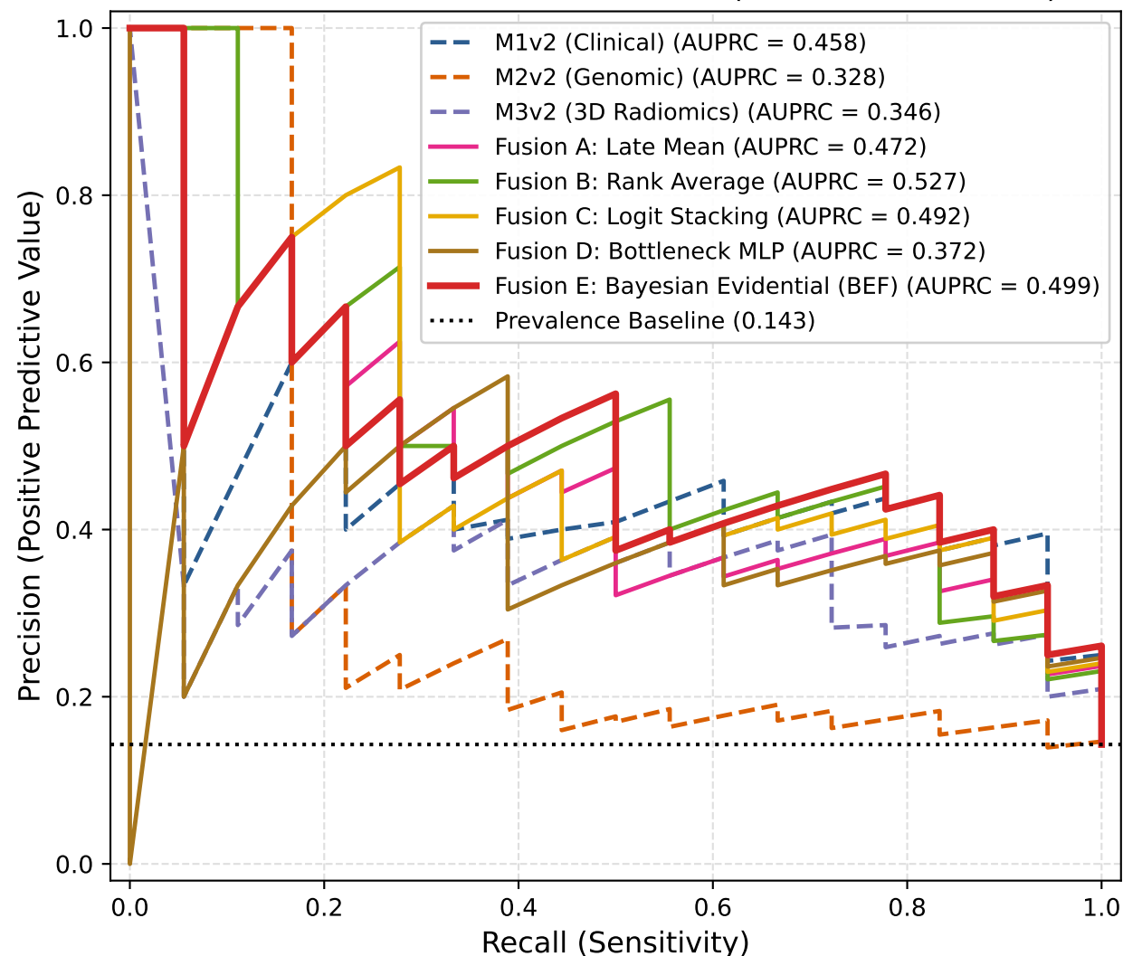
Out-of-Fold Precision-Recall Curves (5-Fold Stratified CV)
