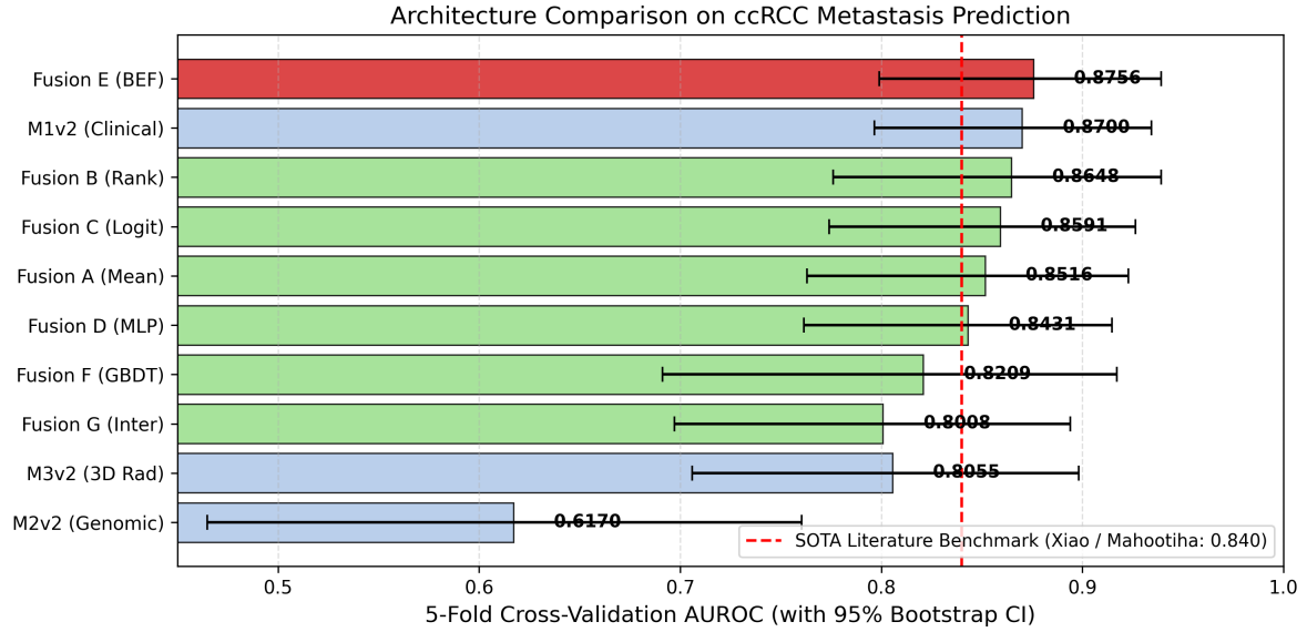
Figure 3: Comparative 5-fold cross-validation AUROC performance with 95% bootstrap confidence intervals across architectures, benchmarking against literature standards (0.840).
