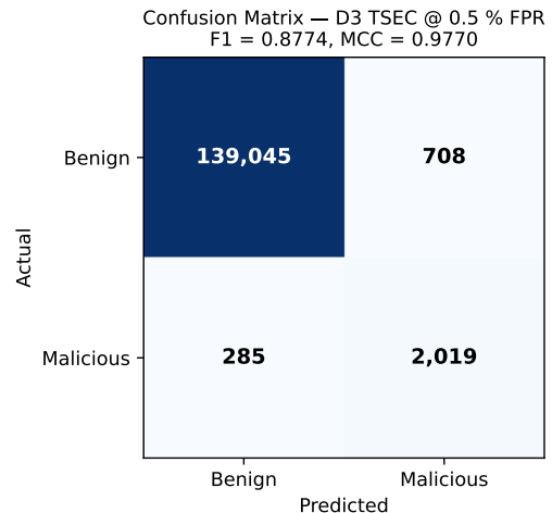
Figure 5: Confusion Matrix: D3 TSEC @ 0.5% FPR (F1 = 0.8774, MCC = 0.9770).
