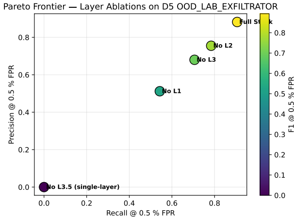
Figure 7: Pareto Precision-Recall Frontier Across Layer Ablations on D5 Hold-Out.
