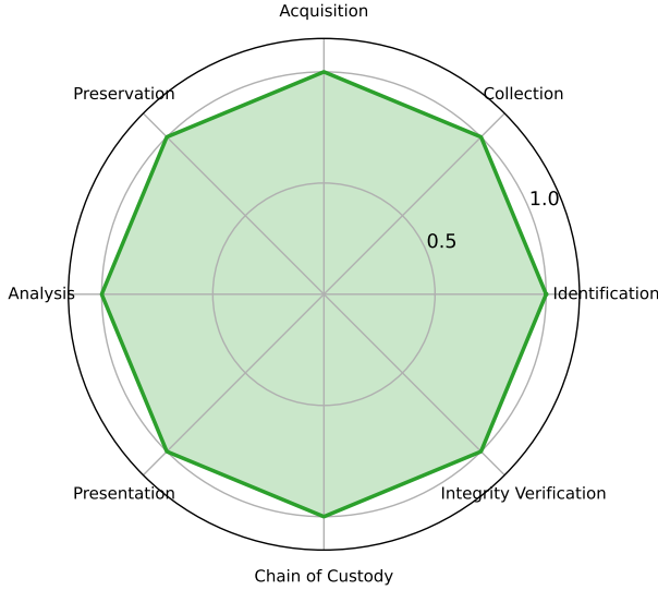
ISO/IEC 27043 Attribute Coverage — 100 % (all 8 attributes)
