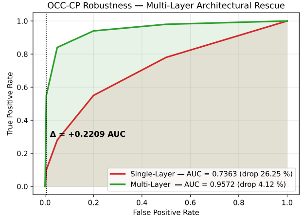
Figure 8: OCC-CP Robustness: Multi-Layer Architectural Rescue Overlay.
