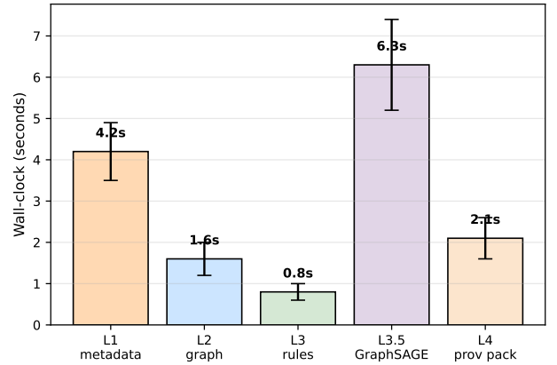
Figure 10: Wall-Clock Decomposition per 1 K Activity Records.
